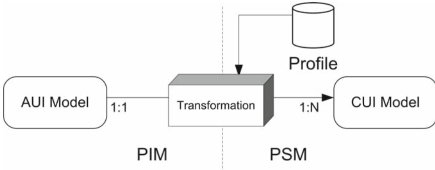
Fig. 4.1 AUI model to CUI model transformation using a Transformation Profile
