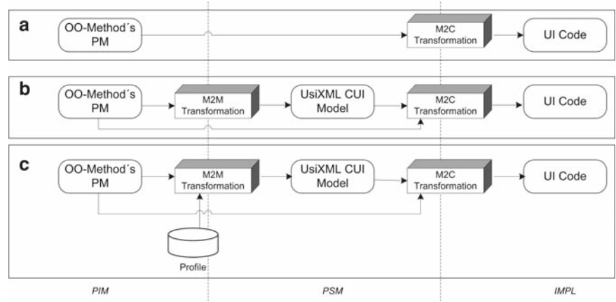
Fig. 4.3 OO-Method UI generation process: (a) in its current state, (b) as proposed in [11], and (c) using a Transformation Profile
