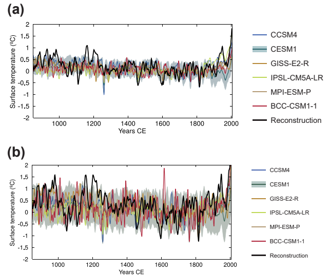
Figure 1. Summer temperature averaged over (a) Europe and (b) the Alpine region (defined here as the area between 45 and 48° N and between 6 and 13° E) in the reconstruction of Luterbacher et al. (2016) and as simulated by climate models over the past millennium. The shaded area represents the mean plus and minus 1 standard deviation of the CESM1 model ensemble. A 15-year Lowess smoothing has been applied to the time series. The reference period is the years 1500–1850 CE as in Luterbacher et al. (2016).
