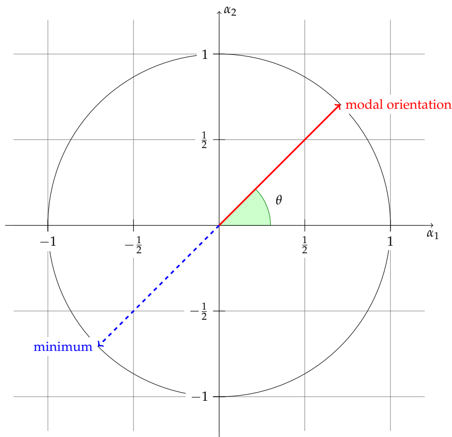
Figure 2. Stiefel manifold for p = 2 and r = 1 .
