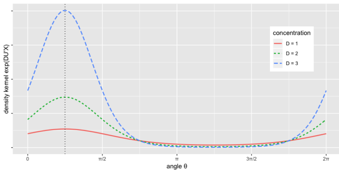
Figure 3. Matrix Langevin density kernels for p = 2 and r = 1 .
