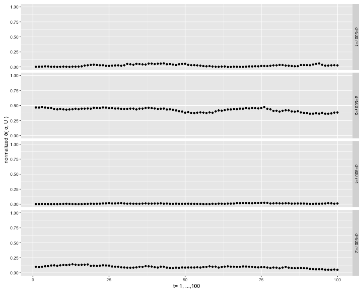
Figure 8. Normalized distances \delta_t for the settings p = 3 , r \in \{1, 2\} , \rho = 0.1 and d = \{500, 800\} .
