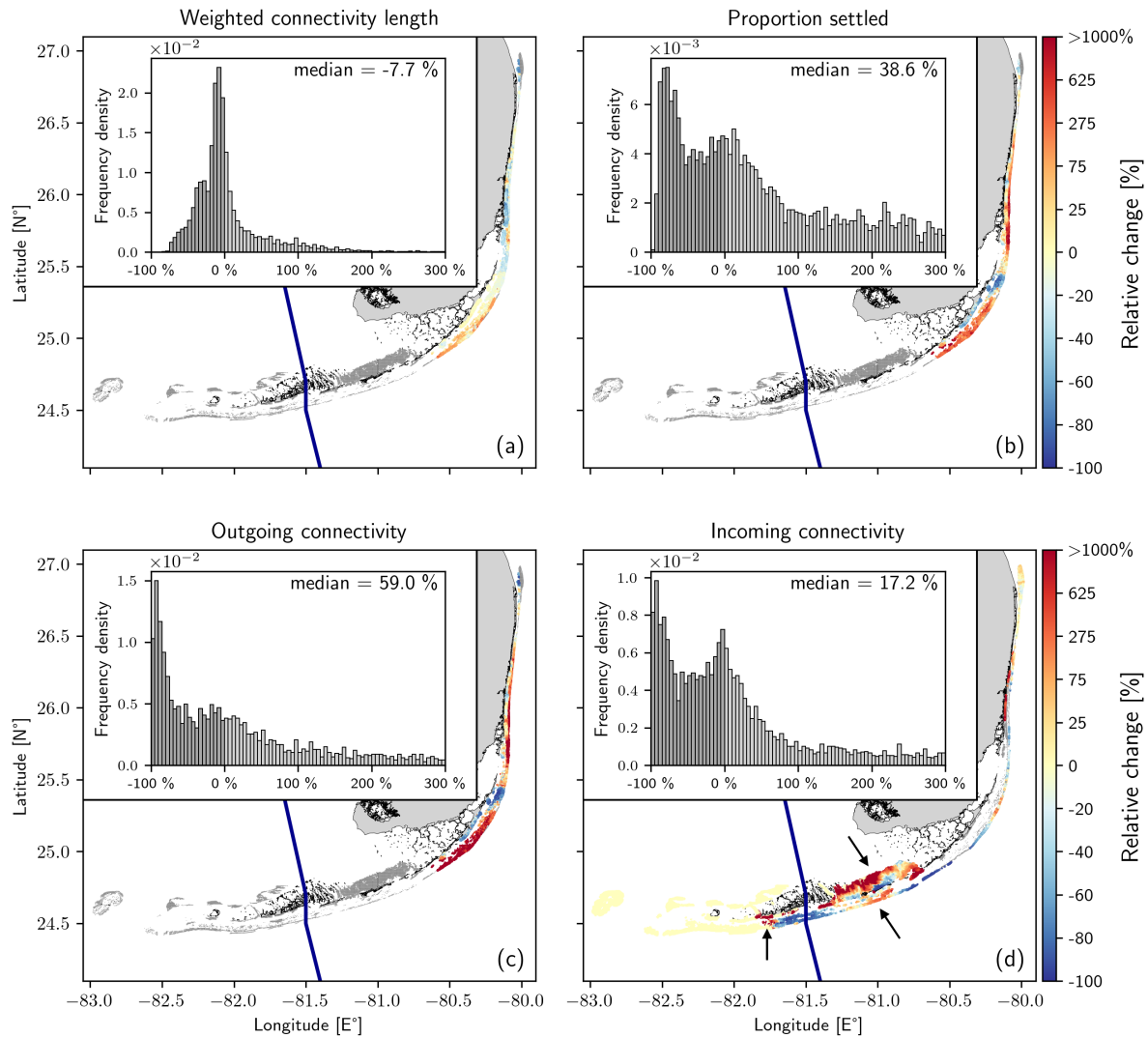
Figure 4. Same as Fig. 3 for disease dispersal. Note that the zero values in panel (d) west of the Lower Keys correspond to reefs for which there is no incoming connectivity both with and without Irma. The relative change is thus undefined and they are not considered in the frequency density histogram. Arrows in panel (d) highlight patches of susceptible reefs that experienced a surge in incoming disease connectivity following the passage of Irma.
