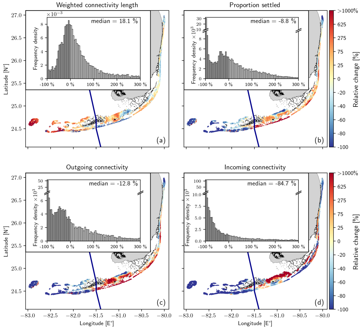
Figure 3. Spatial distributions alongside frequency density histograms illustrating the relative changes induced by Hurricane Irma in larval (a) weighted connectivity length, (b) proportion settled, (c) outgoing connectivity, and (d) incoming connectivity. The trajectory of Hurricane Irma is depicted by a solid blue line. The horizontal axis of the histograms has been cropped to 300% to improve readability.
