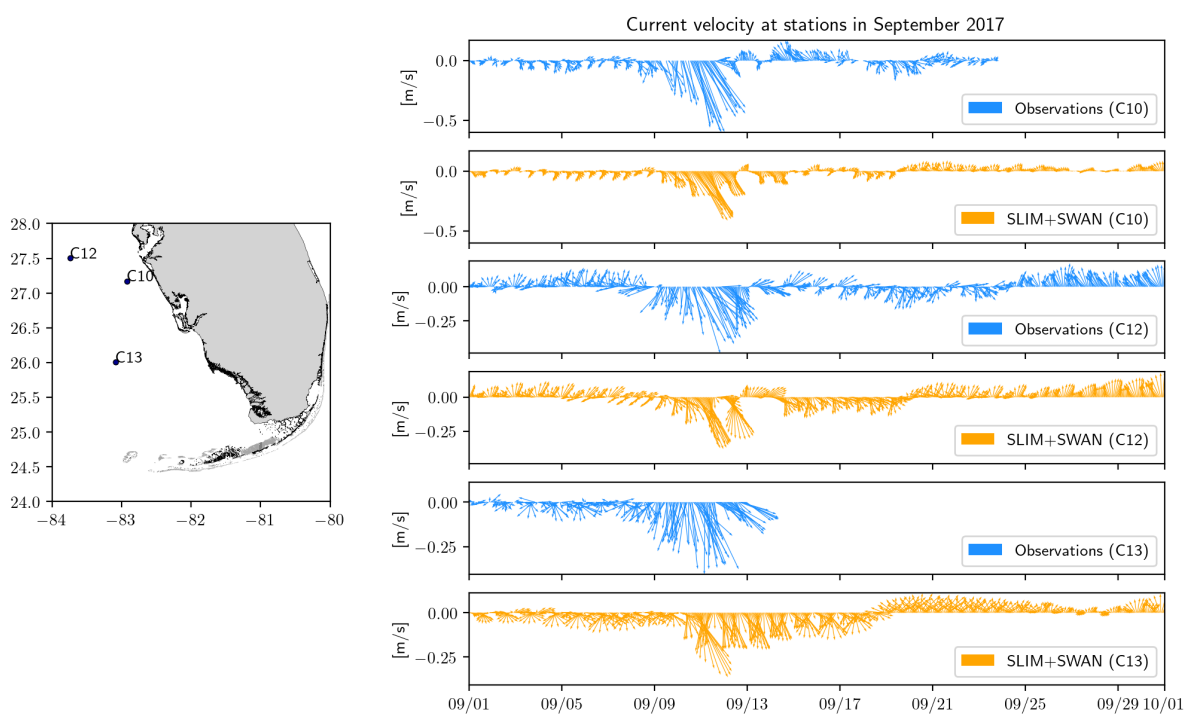
Figure 6. Validation of model outputs against ADCP current velocity measurements in September 2017
