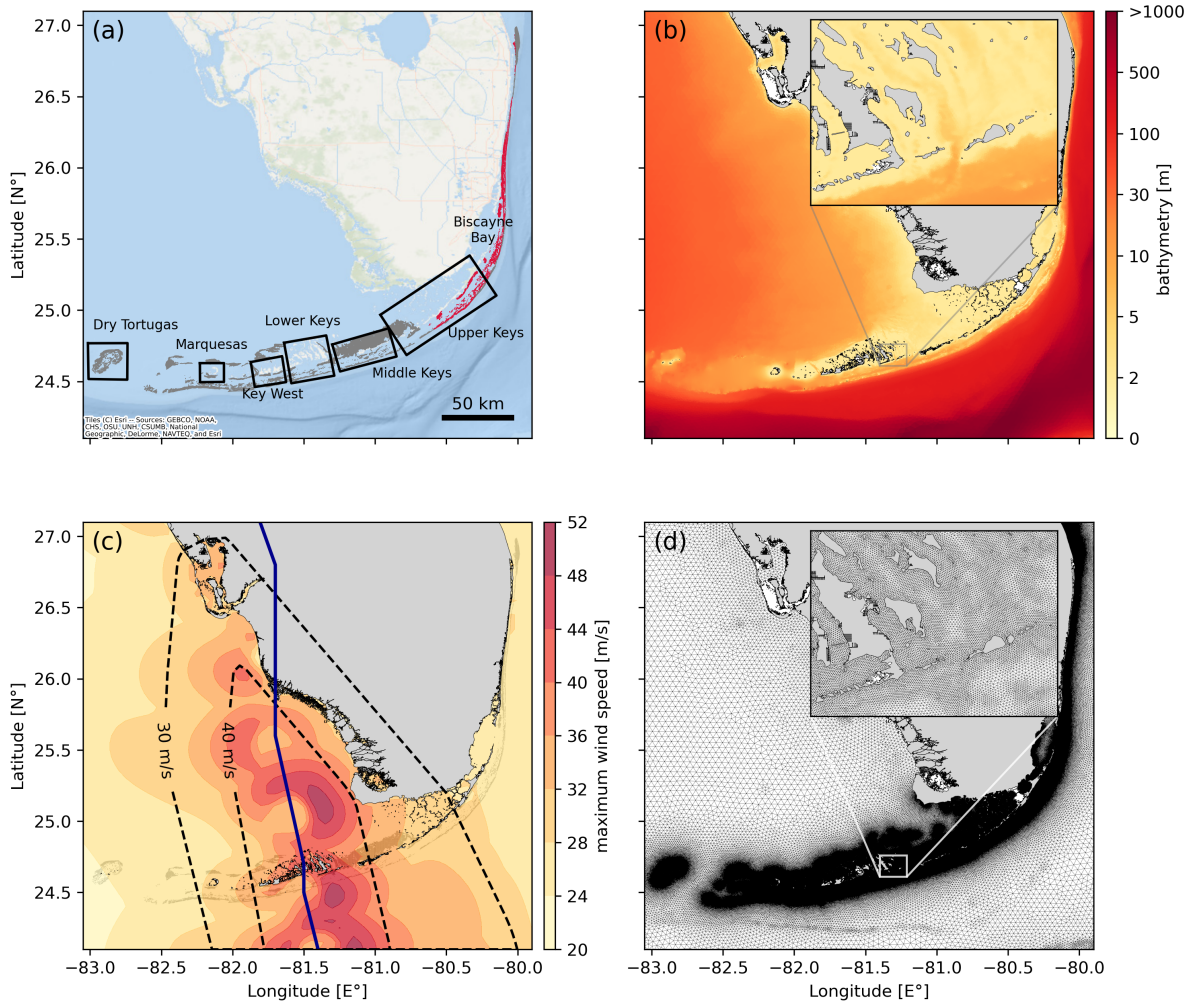
Figure 1. Overview of the area of interest with (a) Florida's Coral Reef with healthy/susceptible reefs shown in dark grey and infected reefs shown in red, (b) the model bathymetry, (c) the maximum wind speed during Hurricane Irma (30 m/s and 40 m/s isolines in black dotted lines and track of Irma in dark blue) and (d) the model unstructured mesh whose resolution ranges from \sim 100 m near the coast and reefs in FCR to \sim 5 km offshore.
