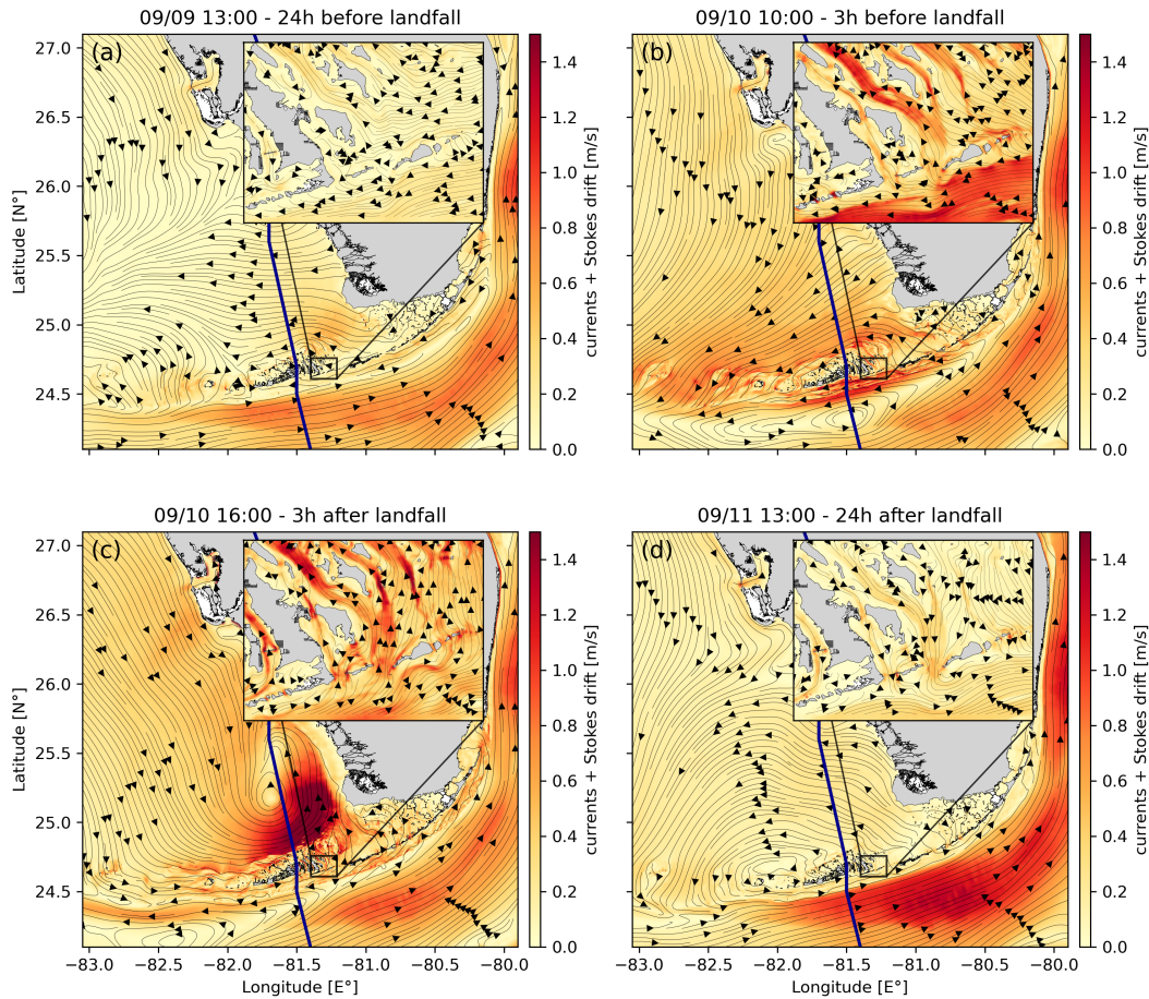
Figure 2. Snapshots of the combined modeled depth-averaged currents and Stokes drift (a) 24h before landfall, (b) 3h before landfall, (c) 3h after landfall and (d) 24h after landfall. Note strong westward current developing offshore of the Lower Keys in panel (b). The trajectory of the hurricane is depicted by a solid blue line.
