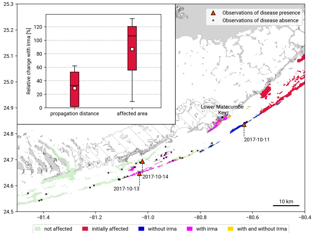
Figure 5. Propagation of the disease simulated by the connectivity-based epidemiological model between Sept. 1 and Dec. 1 2017 using the reference (dark blue) and hurricane (magenta) connectivity matrices. Reefs affected by SCTLD prior to Sep 1 2017 are shown in red and fully susceptible reefs in green. Vaca Reef , which was filtered out of the connectivity matrices, is represented by a hashed white polygon. Observations of disease presence and absence between the landfall of Irma and Dec. 1 2017 are respectively shown by red triangles and black crosses. These observations were extracted from (i) Coral Reef Evaluation and Monitoring Project (CREMP; 2014–2017), (ii) CREMP Presence/Absence Data (CREMP P_A; 2016–2017), (iii) Southeast Florida Coral Reef Evaluation and Monitoring Project (SECREMP; 2014–2017), (iv) Florida Reef Resilience Program Disturbance Response Monitoring (FRRP; 2014–2017), (v) Hurricane Irma Rapid Reef Assessment (IRMA; 2017), (vi) the Southeast Florida Action Network citizen science program (SEAFAN; 2014–2017), and (vii) the Southern Coral Disease Margin field effort (2017 and 2018). The upper left graph shows the relative change in the distance travelled by the disease front and the total affected area when accounting for Irma for different values of the model’s infection threshold. The central lines of the boxes and the white square respectively indicate the median and mean of the relative change, the bottom and top of the boxes indicate the 25th and 75th percentiles respectively, while the minimum and maximum of the relative change are indicated by the bottom and top whiskers. On average, the hurricane caused a 28.9% increase in disease propagation distance and an 87.0% increase in affected area, equivalent to about 25 days of disease propagation under fair weather conditions.
