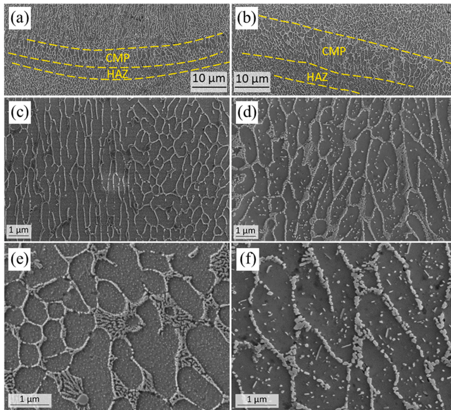
Fig. 14. Influence of build platform temperature on microstructure of LPBF AlSi10Mg [26]. Melt pool border (a), Si-rich network (c) and nanosized particles (e) in 35^{\circ}\text{C} case, melt pool border (b), Si-rich network (d) and nanosized particles (f) in 200^{\circ}\text{C} case. The figures are reproduced with permission from Elsevier.
