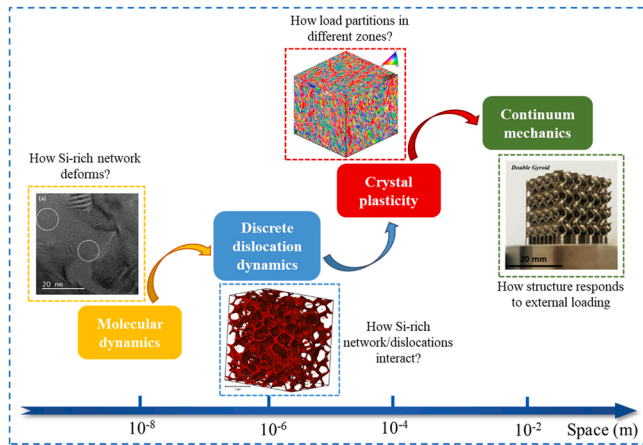
Fig. 49. Multiscale modeling and simulation strategy for LPBF AlSi10Mg. The inserted figures are reprinted from [25,26,73,92] with permission from Elsevier.
