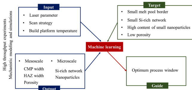
Fig. 46. Machine learning assisted process optimization workflow.
