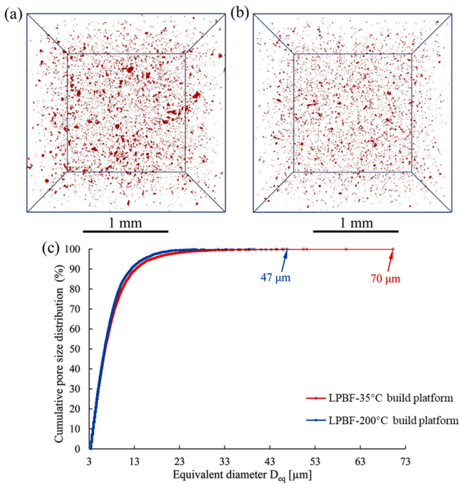
Fig. 19. 3D tomographies showing the porosity of LPBF AlSi10Mg manufactured using machine manufacturer suggested parameters (EOS M290) with a slight build platform preheating to 35 °C (a) and a build platform preheating to 200 °C (b), cumulative pore size distribution based on the data of (a) and (b) (c) [38].
