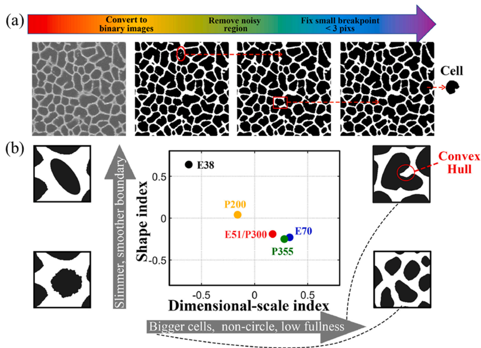
Fig. 47. Definition of dimensional-scale index I_d and shape index I_s [68]. Image processing steps to extract the Si-rich network (a), schematic interpretation for mean values of the morphology indices I_d and I_s (b). The figures are reprinted with permission from Elsevier.
