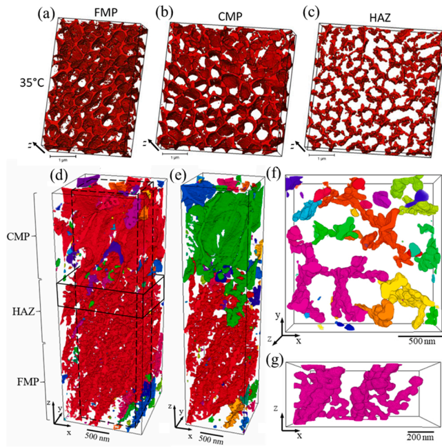
Fig. 10. FIB/SEM tomographies for the three distinct zones in an LPBF AlSi10Mg sample built with 35 °C build platform (the z axis corresponds to the building direction). Si-rich eutectic network of separate FMP (a), CMP (b) and HAZ (c), 3D rendering of Si-rich eutectic across the melt pool border (d) and a subvolume of (d) (e), local 3D views of HAZ along the building (f) and transverse (g) directions.
