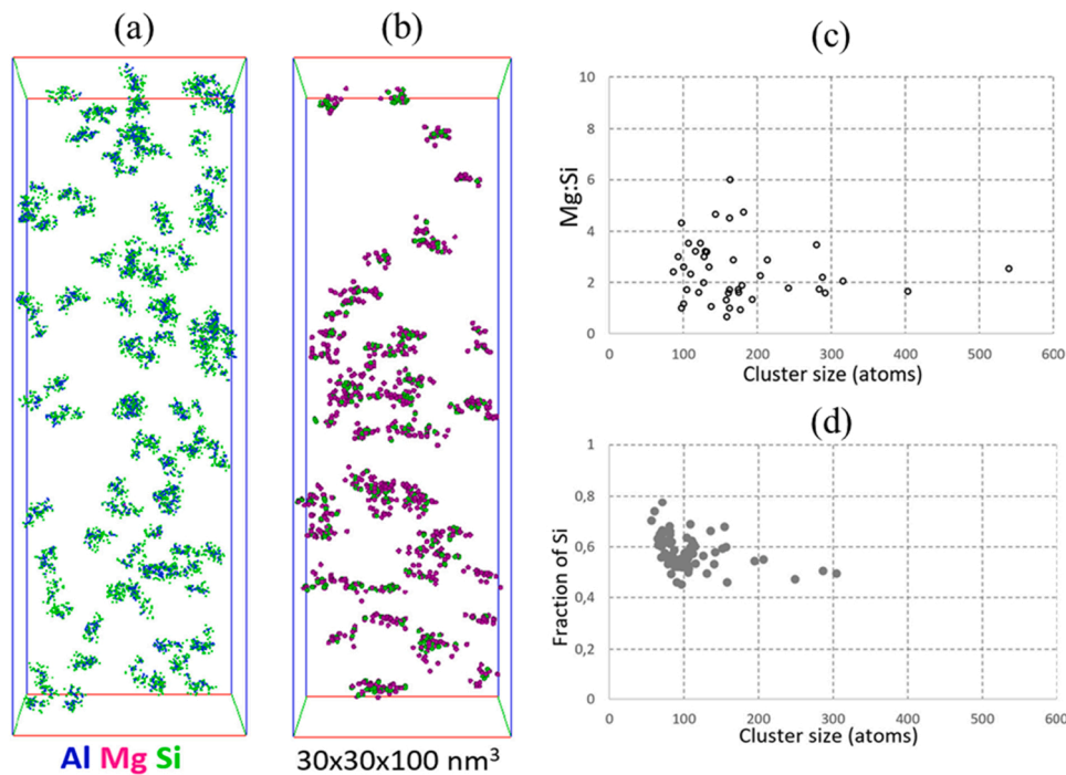
Fig. 4. Supersaturated Si and Mg atoms in Al matrix viewed by APT [25]. Si-rich atom clusters (a), Mg-rich atom clusters (b), Mg: Si ratio in clusters in (b) (c), fraction of Si in clusters shown in (a) (d).
