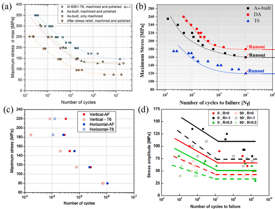
Fig. 37. Fatigue life of as built LPBF AlSi10Mg. Comparison with Al 6061-T6 and stress relief state [52] (a), comparison with direct aging and T6 states [198] (b), comparison between horizontal and vertical samples [65] (c), comparison between different stress ratios and loading directions [199] (d). DA means direct aging in (b), AF means as fabricated in (c), 0^\circ and 90^\circ correspond to horizontal and vertical samples, respectively, in (d). The figures are reprinted with permission from Elsevier.
