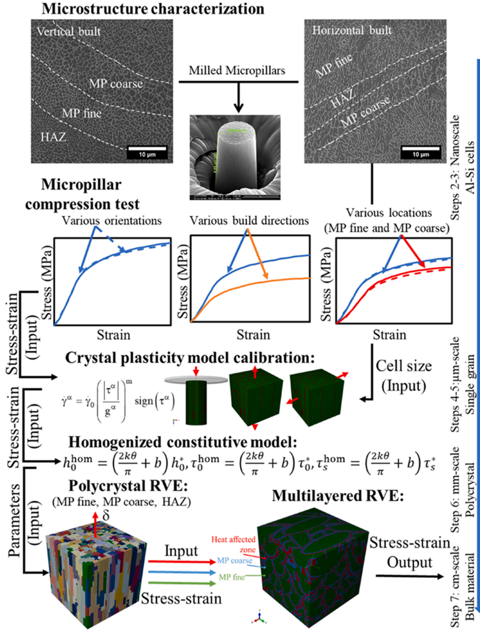
Fig. 44. Microstructure based multi-scale crystal plasticity modeling scheme of LPBF AlSi10Mg [182].
