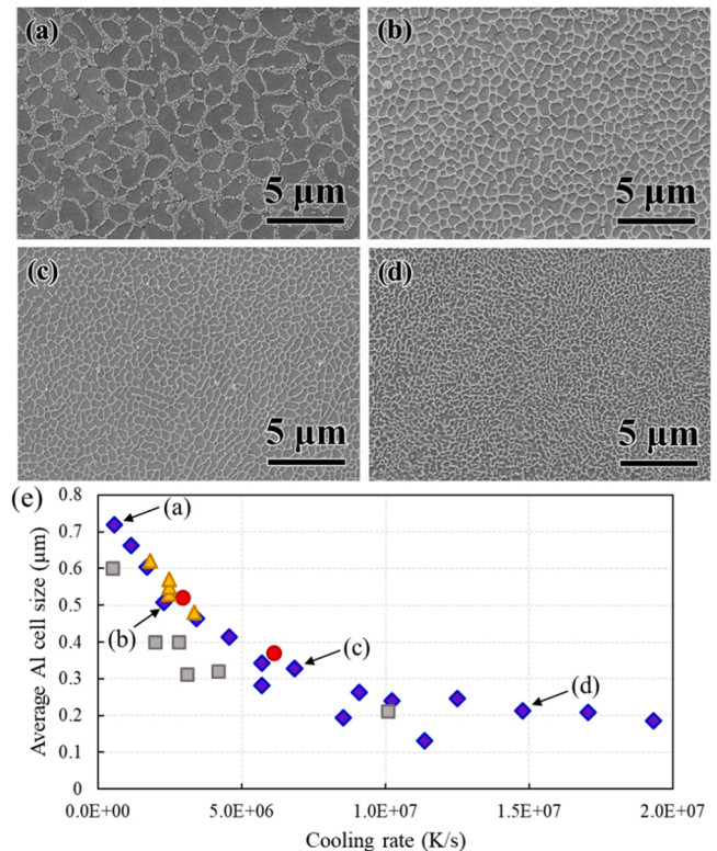
Fig. 13. Effect of cooling rate on Al cell size. SEM micrographs of Al cell structures [107] with a scan speed of 100 mm/s (a), 400 mm/s (b), 1200 mm/s (c) and 2600 mm/s (d) at fixed laser power (250 W), layer thickness (30 \mu m), hatch spacing (0.13 mm) and build platform temperature (100 ^{\circ} C), relationship between average Al cell size and cooling rate calculated with Eq. (1) at fixed layer thickness and hatch spacing (e). The symbols of diamond, square, circle and triangle represent data from Refs [26,106,107] and [68], respectively. The corresponding cooling rates for (a)-(d) are marked in (e). The figures are reproduced with permission from Springer Nature.
