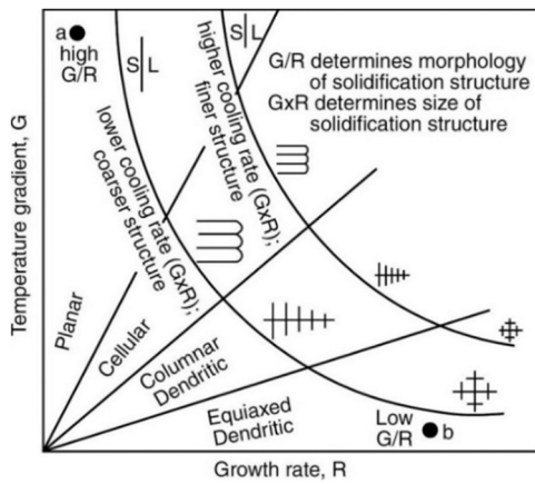
Fig. 12. Effect of temperature gradient G and growth rate R on the morphology and fineness of the solidification structure [78]. The figure is reprinted with permission from Elsevier.
