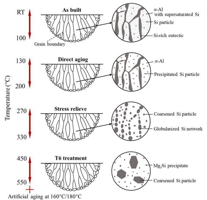
Fig. 15. Influence of post-printing heat treatment on microstructure of LPBF AlSi10Mg.
