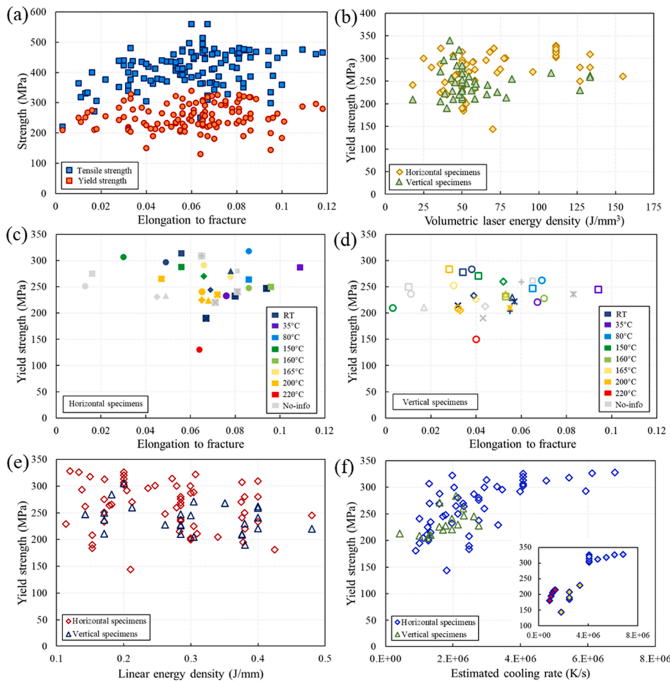
Fig. 20. Statistics on tensile properties of as built LPBF AlSi10Mg based on data reported in literature. Strength vs. elongation to fracture (a), yield strength vs. volumetric laser energy density (b), yield strength vs. elongation to fracture with different build platform temperatures for horizontal specimens (c) and vertical specimens (d), yield strength vs. linear energy density (e), yield strength vs. estimated cooling rate (f). Horizontal specimens involve loading direction perpendicular to building direction while vertical specimens involve loading direction parallel to building direction. The data points are collected from Refs [27,31,36–38,40, 41,43–46,49,52,55,62,64,65,68,81,88,91,93, 110–120,123,125,127,146–159]. The inset in (f) shows three individual studies (from left to right [159], [68], [155]) where the effect of cooling rate on yield strength of horizontal specimens can be observed.
