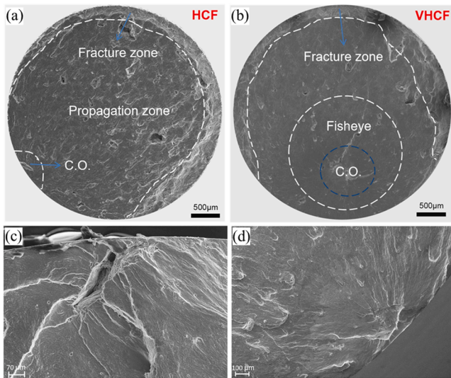
Fig. 38. Fatigue crack origins of as built LPBF AlSi10Mg samples. Surface porosity in high cycle fatigue with N = 2.74 \times 10^6 (a), internal porosity in very high cycle fatigue with N = 4.48 \times 10^8 [37] (b), typical manifestation of fracture origin (lack of fusion defects) for horizontal (c) and vertical (d) samples [118]. C.O. in (a) and (b) represents crack origin. The figures are reprinted with permission from Elsevier.
