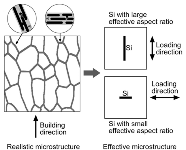
Fig. 31. Schematic drawing of effective aspect ratio of the Si-rich network for horizontal and vertical specimens [185].
