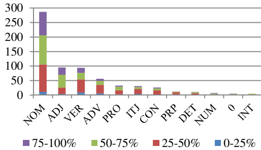
Figure 3. Boundary force / POS tag
