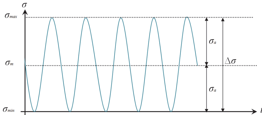
Figure 3: Tensile repeated solicitation on fatigue test.
