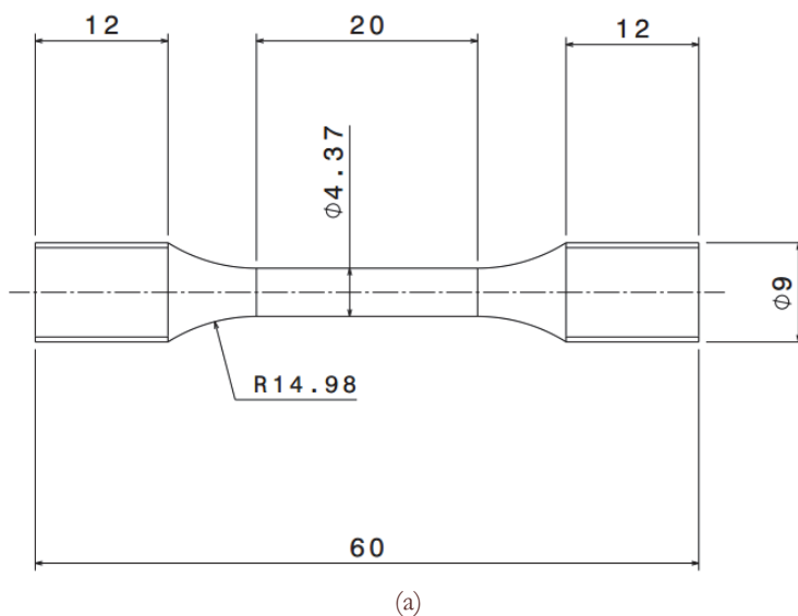
Figure 1: Fatigue specimen (a) schematic illustration showing the specimen geometry and (b) image of the actual fatigue specimen.
