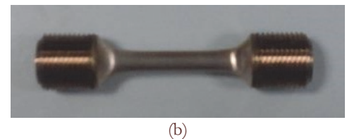
Figure 1: Fatigue specimen (a) schematic illustration showing the specimen geometry and (b) image of the actual fatigue specimen.
