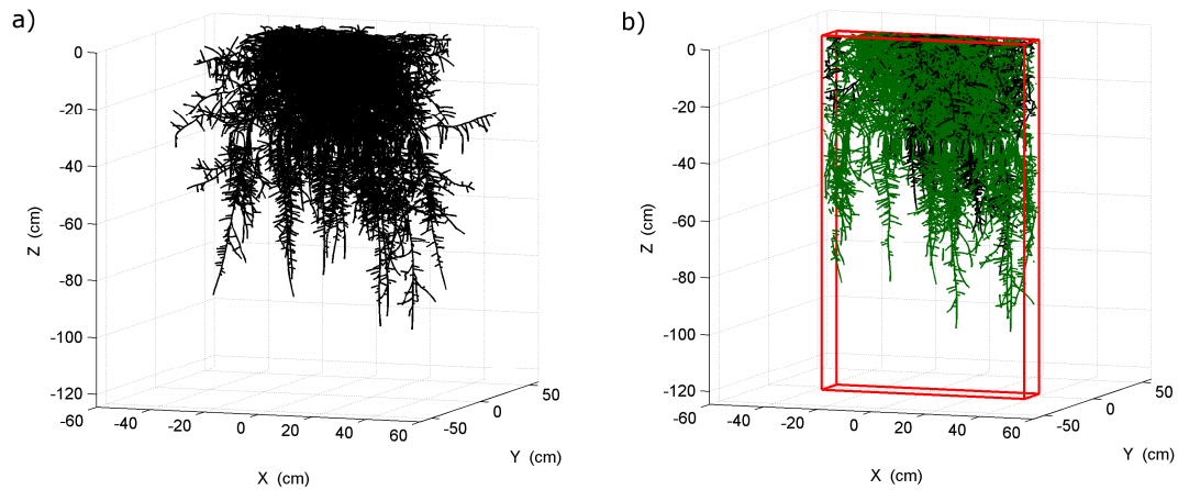
Fig. 2. Optimised 80-days old maize root system architecture (a) fully deployed and (b) in the periodic domain, green roots having crossed the domain boundaries (red).
