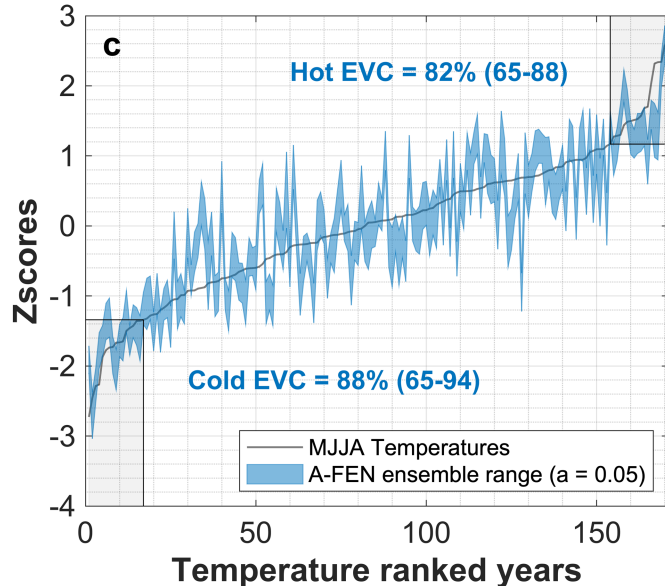
Extended Data Fig. 1 | Evaluation of the ability of the A-FEN and X-FEN reconstructions to capture extremes in climate targets. The instrumental temperature data was sorted from coldest to warmest and plotted together with the reconstruction values of the corresponding years. The grey boxes are bound by the 10% coldest and warmest years, and the 10 th and 90 th percentile of the zscore temperatures, respectively. If an extreme reconstruction value is found within the grey box, the extreme is defined as “captured”. The sum of the captured values divided by the potential sum of values, is calculated and presented as a percentage of extreme value capturing (EVC). In McCarroll, et al. 21 , a significance testing was implemented, and for 160–170 years of climate data, p < 0.001 is achieved if more than 40% of values are captured. a) A-FEN’s ability
