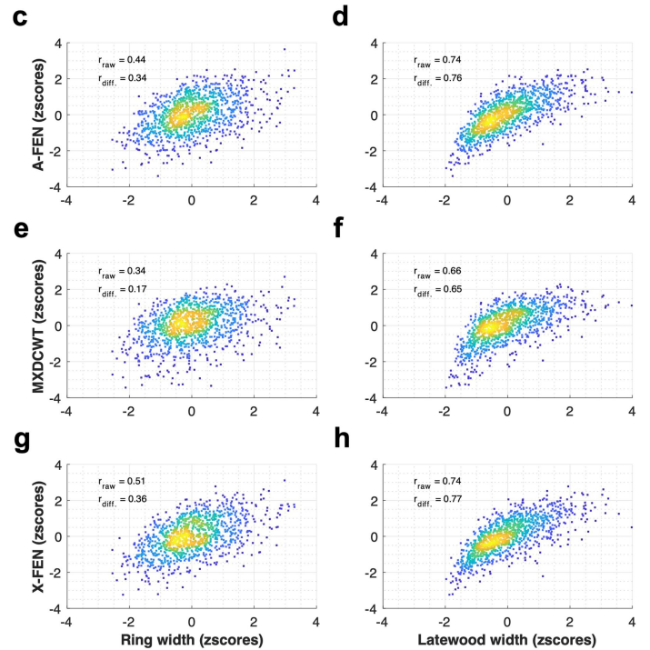
associated with comparatively lower MXD values even though the “true” MXD value may be high. c) Relationships between TRW and A-FEN and d) LWL and A-FEN. e) Relationships between TRW and anatomical MXD (MXDCWT) and f) LWL and MXDCWT. g) Relationships between TRW and X-FEN and h) LWL and X-FEN. All datasets display correlations and using datapoints covering 850–2005 CE. Note how the X-FEN always is stronger correlated with TRW and LWL than the MXDCWT. A higher correlation is expected if TRW or LWL is affecting the measurement. Spearman rank correlation coefficients were used due to the possibly non-linear relationships between width and density. r_{\text{raw}} and r_{\text{diff}} refers to untreated and first differenced data prior to correlations, respectively.
