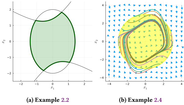
Figure 1: (a) The BSA set in Example 2.2 (green area). (b) Vector field (blue arrows), initial set (yellow area) and sample trajectories (colored curves) of the system in Example 2.4.
