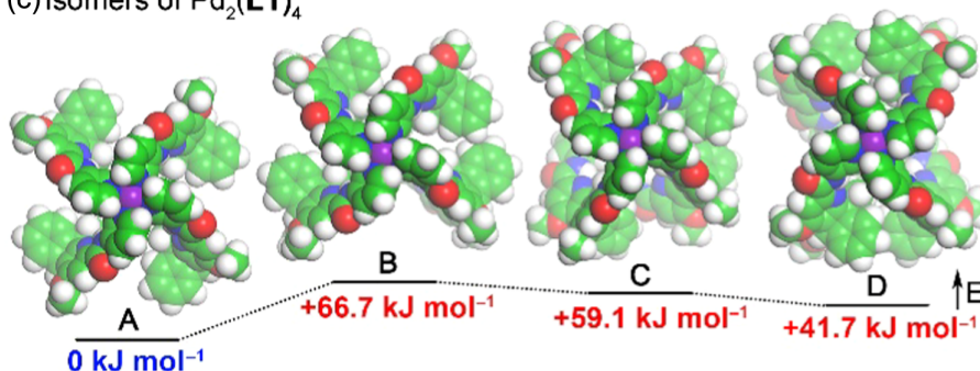
Figure 3 | DFT-calculated structures and relative energies (B3LYP/6-31g* for ligands and B3LYP/def2SVP for cages) of (a) three possible conformations of ligand L1 ( L1A , L1B and L1C ), (b) \text{Pd}_2(\text{L1})_4 cage with representative ligand syn/anti amide conformations, and (c) four possible diastereomers of \text{Pd}_2(\text{L1})_4 cage based on triptycene orientation.
