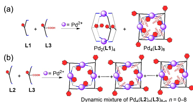
Figure 7 | Mixed ligands self-assembly with ligand L3 , mixed with (a) L1 leads to narcissistic self-sorting of M 2 ( L1 ) 4 and M 4 ( L3 ) 8 assemblies and (b) L2 formed nonsorted scrambled dynamic mixtures of Pd 4 ( L2 ) n ( L3 ) 8-n (BF 4 ) 8 , n = 0–8.
