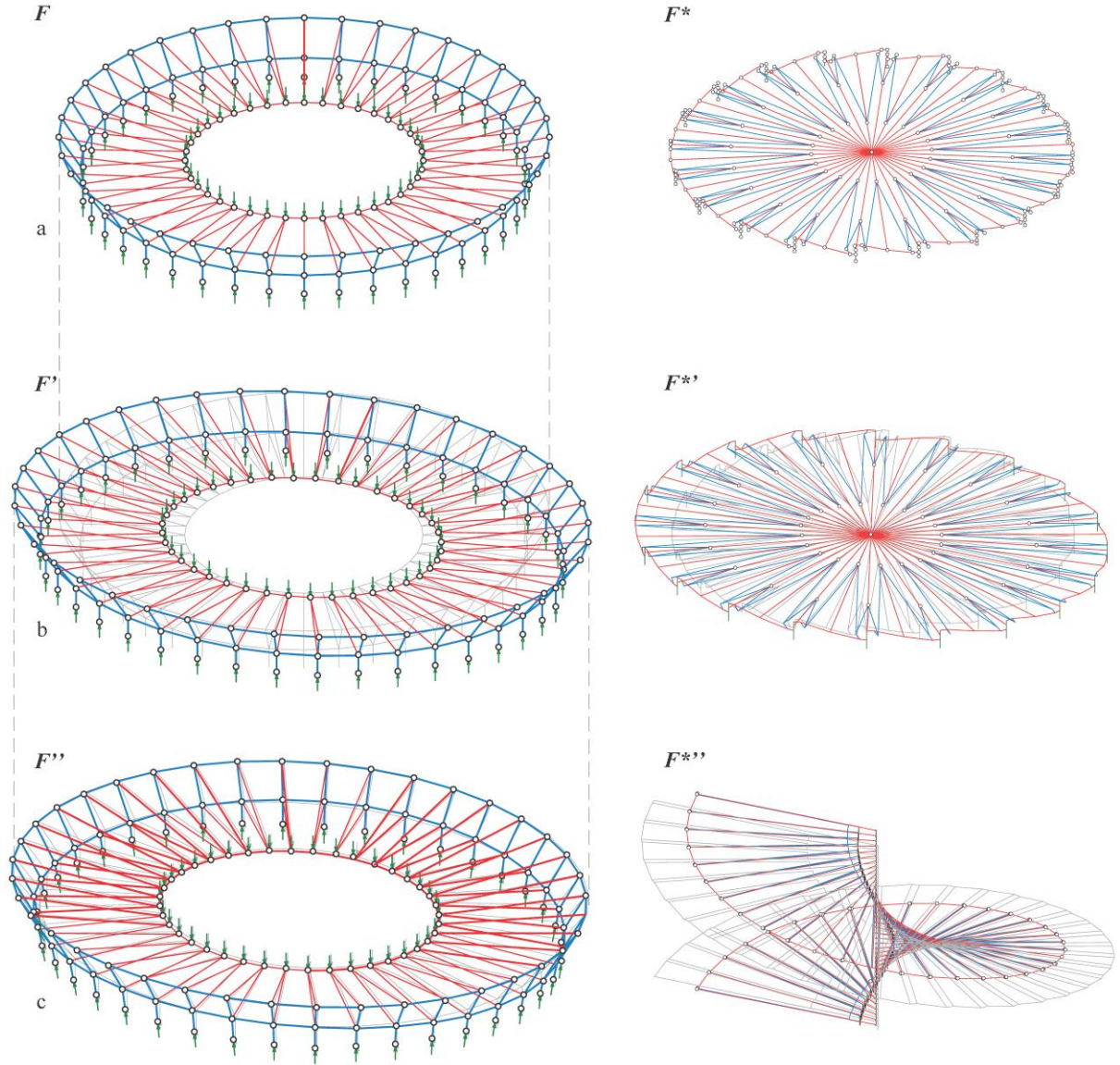
Figure 17: Conceptual design of a spoked wheel stadium roof: (a) initial equilibrium state based on form F and force F^* diagrams; (b) equilibrium state after global transformations of F and F^* (in grey) into F' and F^{*'} (in colours); (c) equilibrium state after local transformations, leading to the final form F'' and force F^{*''} diagrams (in colours); note that in this case a topologically different force diagram configuration is adopted in comparison to the one used in the previous steps.
