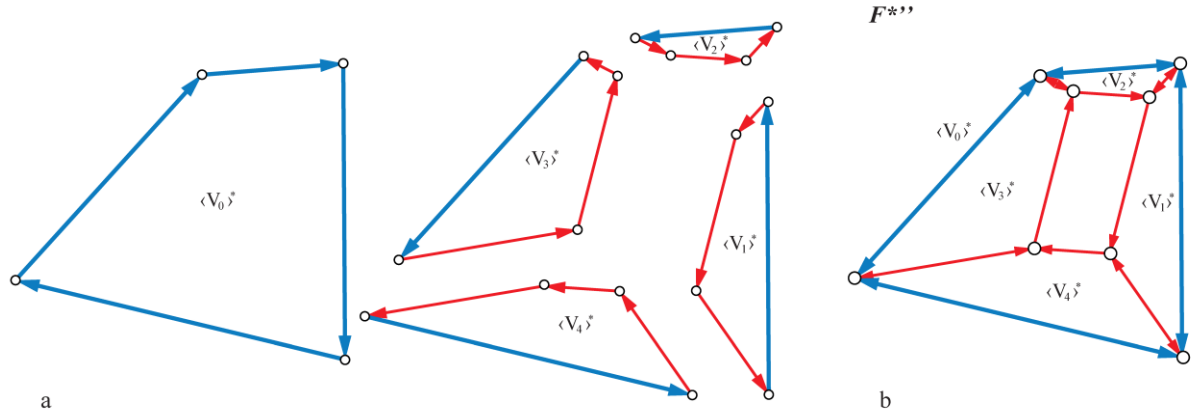
Figure 2: (a) individual closed cycles of force vectors representing the static equilibrium of each node in the self-stressed tetrahedron of Figure 1a; (b) assembly of the cycles shown in (a); note that two pairs of vectors are not overlapped.
