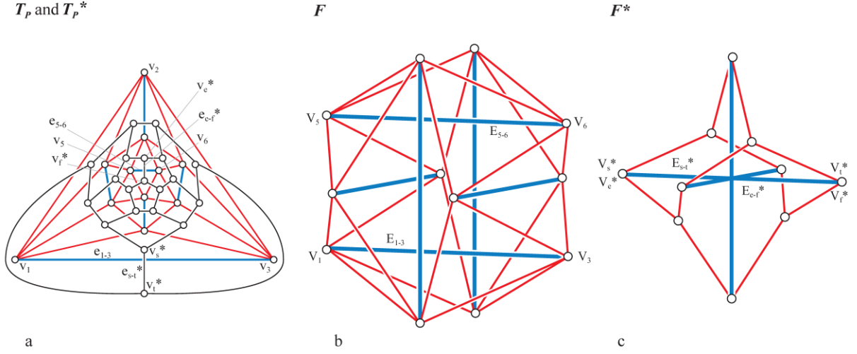
Figure 4: (a) Plane graph T_P of a Jessen's icosahedron and its dual T_P^* ; (b) 3D form diagram F of the Jessen's icosahedron; (c) reciprocal 3D force diagram F^* : if regarded as the 3D form diagram of a structure with all duplicated elements, F is its reciprocal force diagram.
