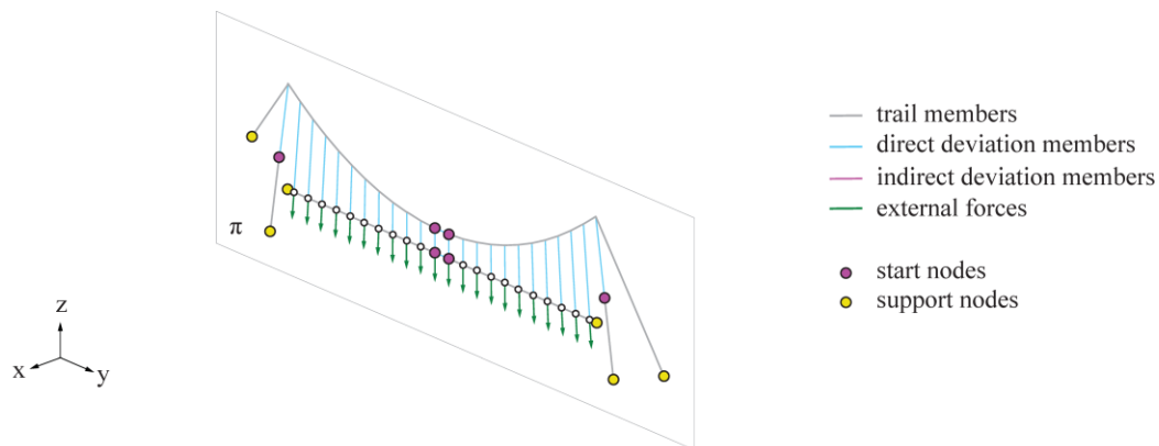
Figure 13: Conceptual design of a pedestrian bridge: initial set-up for the form-finding
