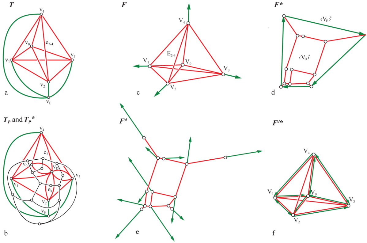
Figure 7: (a) Graph T of an externally loaded self-stressed tetrahedron; (b) plane graph T_p with one additional vertex v_D and its dual T_p^* ; (c) vector-based 3D form diagram F ; (d) force diagram F^* with two auxiliary cycles of force vectors \langle v_E \rangle^* and \langle v_D \rangle^* ; (e) F^* regarded as a structure in its own right F^d ; (f) force diagram F^{d*} of F^d assembled as F .
