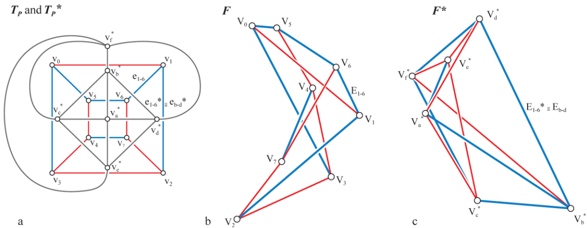
Figure 3: (a) Plane graph T_P (in colours) of a dependent cube and the dual T_P^* (in black) of its reciprocal dependent octahedron; (b) 3D form diagram F of a dependent cube: note that three coplanar edges are incident to each node; (c) reciprocal 3D force diagram F^* : if regarded as a structure in its own right, F^* represents the form diagram of a dependent octahedron, while F is its reciprocal force diagram.
