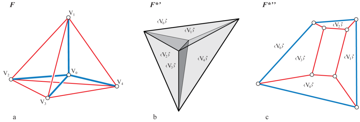
Figure 1: (a) 3D form diagram F of a self-stressed tetrahedron; (b) corresponding polyhedron-based 3D force diagram F^* ; (c) corresponding vector-based 3D force diagram F^{**} .
