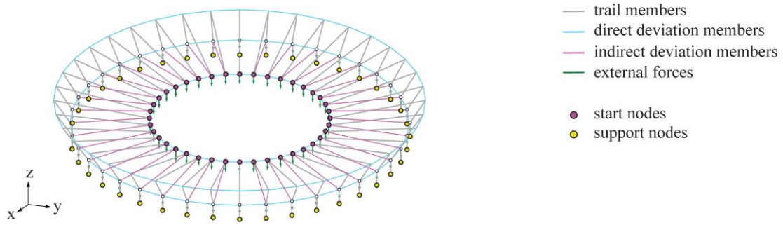
Figure 16: Conceptual design of a spoked wheel stadium roof: initial setup for the form finding
