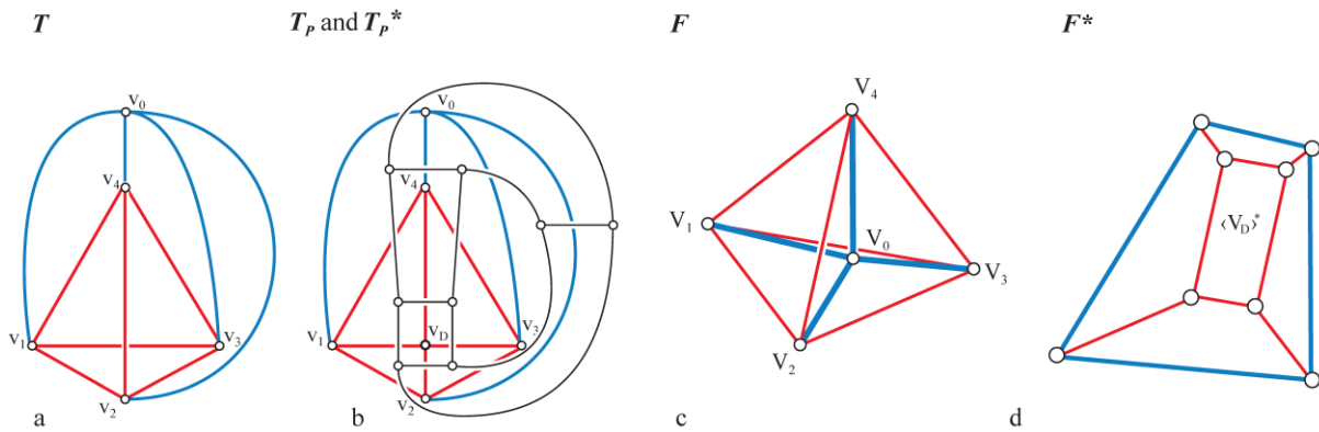
Figure 8: (a) Graph T of a self-stressed tetrahedron; (b) plane graph T_p with one auxiliary vertex v_D and its dual T_p^* ; (c) form diagram F ; (d) force diagram F^* with one auxiliary cycle of force vectors \langle v_D \rangle^* .
