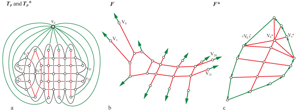
Figure 5: Externally loaded cable-net; (a) plane graph T_P and its dual T_P^* ; (b) 3D form diagram F ; (c) 3D force diagram F^* .
