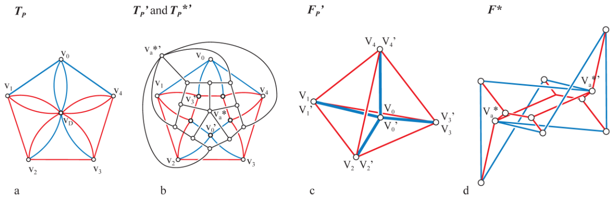
Figure 11: (a) Plane graph \mathbf{T}_P of a self-stressed tetrahedron (Figure 10c); (b) plane graph \mathbf{T}_P' in which all the edges of the initial \mathbf{T} (Figure 10a) are repeated twice, and its dual \mathbf{T}_P^{**} ; (c) vector-based 3D form diagram \mathbf{F}_P'
