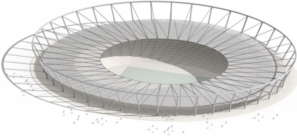
Figure 18: Conceptual view of the stadium roof designed using the proposed vector-based 3D graphic statics framework
