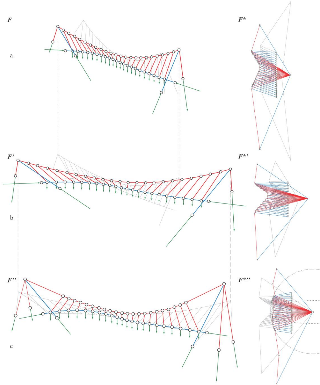
Figure 14: Conceptual design of a pedestrian bridge: (a) initial equilibrium state; (b) equilibrium state after global transformations; (c) equilibrium state after local transformations
