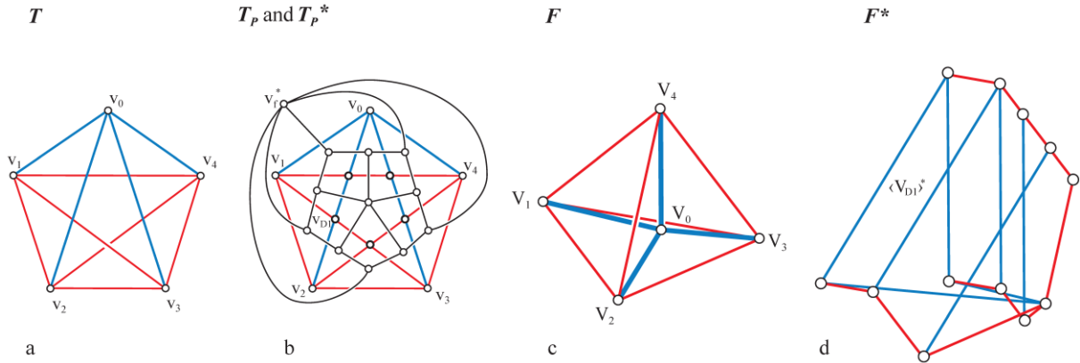
Figure 10: (a) Graph T of a self-stressed tetrahedron; (b) plane graph T_P with additional five extra vertices and its dual T_P^* ; (c) vector-based 3D form diagram F ; (d) force diagram F^* with five quadrilateral cycles \langle V_{Di} \rangle^* corresponding to the auxiliary vertices v_{Di} of T_P .
