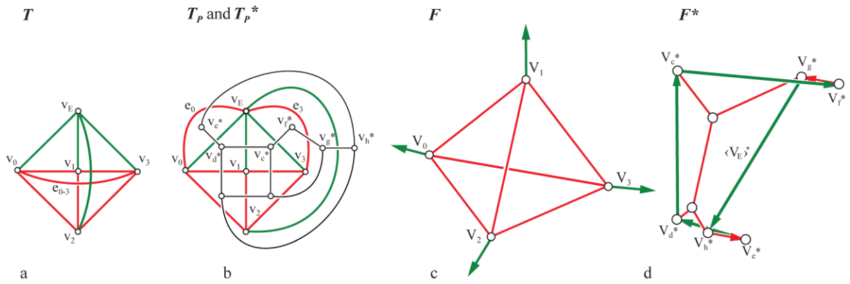
Figure 9: (a) Graph T of an externally loaded tetrahedron; (b) Plane graph T_P with two split edges and its dual T_P^* ; (c) vector-based 3D form diagram F ; (d) force diagram F^* .
