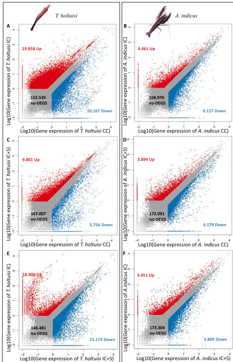
Fig. 4. Differential unigenes expression for Tuleariocaris holthuisi (A; C; E) and Arete indicus (B; D; F). Conditions were “CC: Control condition (with host)”; “IC: Isolation condition”; “IC+S: Isolation condition + spinochromes”. For each comparison (A and B = IC/CC; C and D = IC + S/CC and E and F = IC/IC + S), if fold change >1 = gene(s) is upregulated the first condition compared to the second condition and appears in red, fold change <-1 = gene(s) is downregulated the first condition compared to the second condition and appear in blue, and if fold change is comprised between -1 and +1 = gene(s) is not differentially expressed in the corresponding comparison and appear in grey. The graph was generated using \log_{10} (FPKM +0.01) values.
