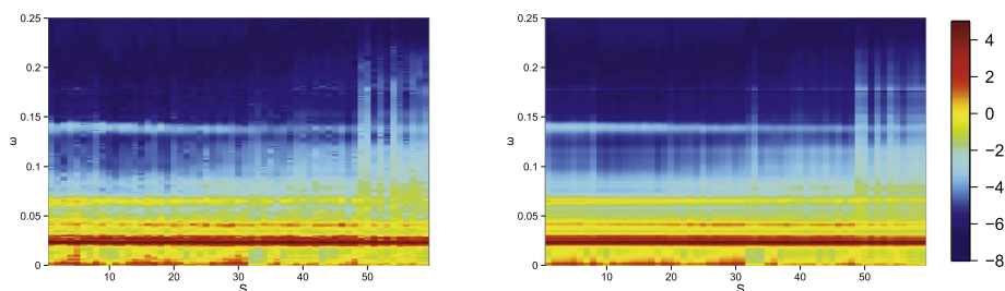
FIG 7. Individually smoothed log-periodograms (left) and predicted trial-specific log-spectra \hat{h}_s^f (right).
