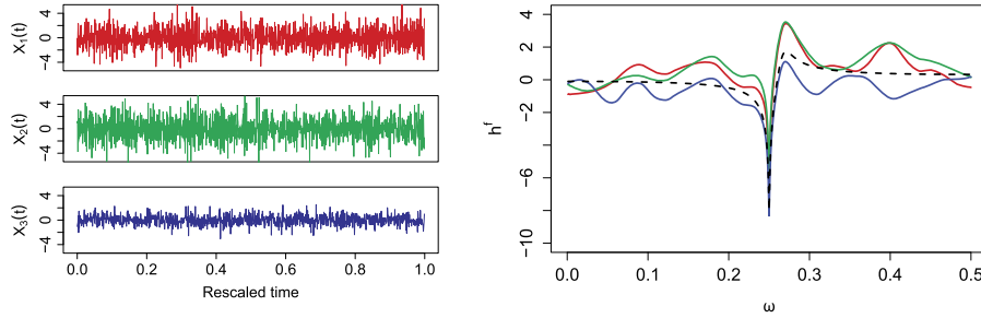
FIG 1. Simulated replicated time series (left), and corresponding replicate-specific log-spectra, with underlying population-mean log-spectrum (right).
