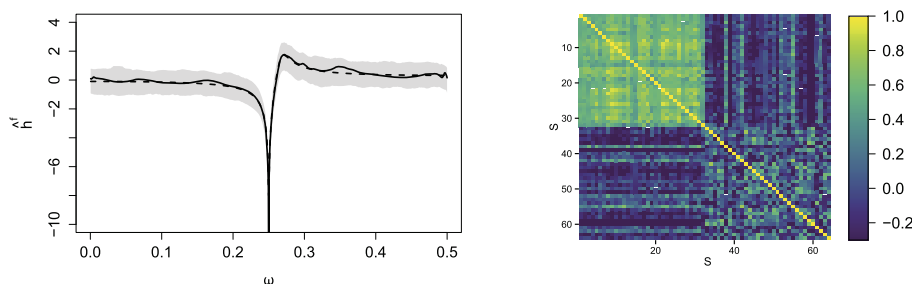
FIG 3. Estimates of \mathbf{h}^f (solid black line) and \mathbf{G}_S for a single simulation experiment, with (\hat{\mathbf{h}}_{0.01}^f, \hat{\mathbf{h}}_{0.99}^f) -empirical pointwise quantiles for 1000 repetitions of the experiment.
