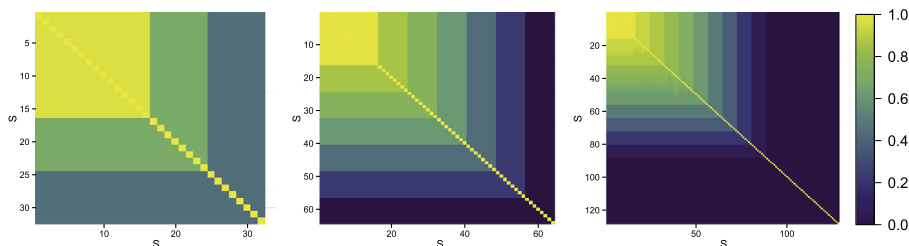
FIG 2. Contour correlation matrices \mathbf{G}_S for S = \{32, 64, 128\} .
