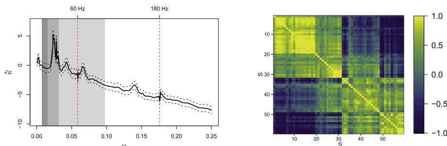
FIG 6. Estimates of the population-mean log-spectrum \hat{h}^f (left) and between-trial correlation matrix G_S (right).
