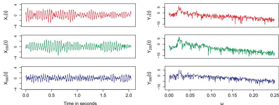
FIG 5. LFP time series (left) and corresponding raw log-periodograms (right) for trials 1, 250, and 590.
