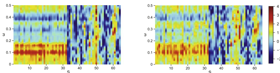
FIG 4. True random effects curves U_s^f(\omega) (left) and predicted random effects curves \hat{U}_s^f(\omega) (right) for a single simulation experiment.
