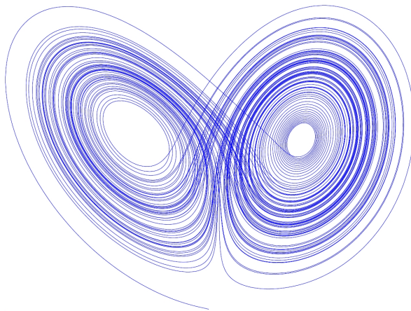
FIGURE 3.1: The strange attractor of Lorenz.
