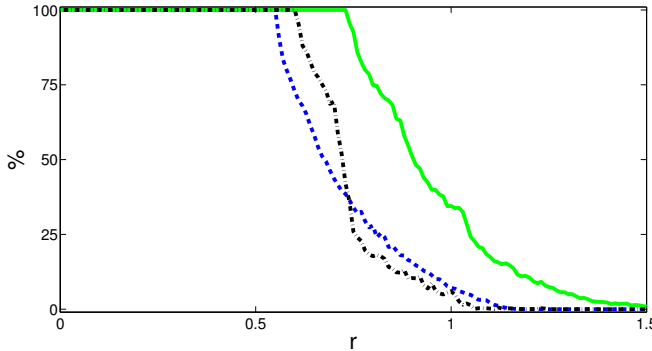
FIGURE 1.7: Percentage of non-escaping orbit versus the distance to the origin. The blue line corresponds to the non controlled map, the green line to the controlled map with the add C_4(F_2) and the black one to the control whose generator is F_{2c} .
