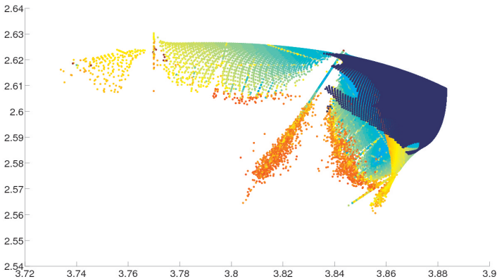
FIGURE 5.18: Frequency space of the (CMo4) : superposition of the results obtained by a normal form approach on those obtained by FMA.
