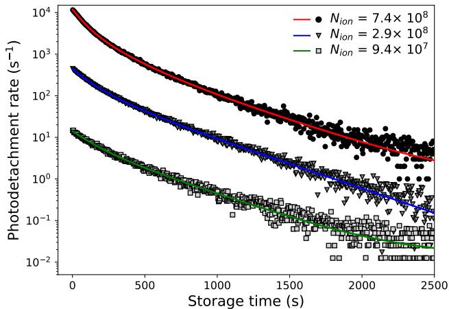
FIG. 4: Photodetachment signals obtained using the Vis laser for three runs with different average numbers of injected ions. For clarity the uppermost and lowermost curves have both been shifted by an order of magnitude, by multiplying them with factors of 10 and 0.1, respectively. The solid lines depict fits to the data. The fit parameters are given in Table IV.
