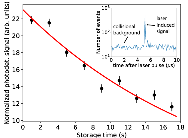
FIG. 8: Background-subtracted normalized photodetachment signal obtained using the pulsed OPO laser. The laser was operated at 2450 nm to photodetach exclusively the weakly-bound ^2P states. The red line shows a single-exponential fit, yielding a lifetime \tau = (22.2 \pm 2.5)\ \text{s} . Inset: Neutral counts as a function of time after the OPO laser pulse.
