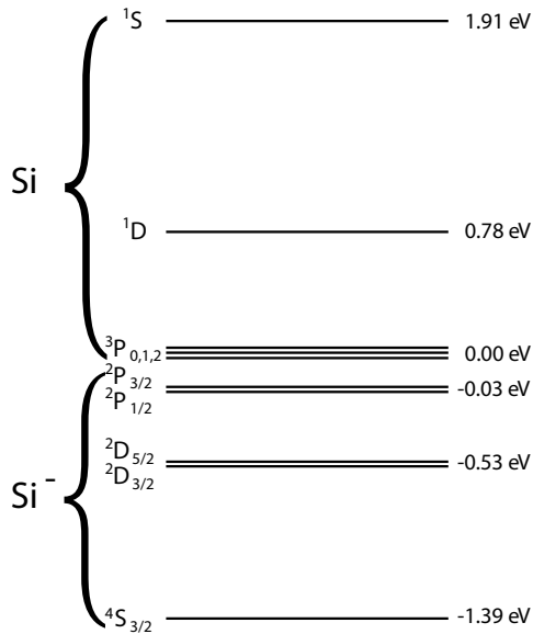
FIG. 1: Level diagram (energy axis not to scale) for \text{Si}^- and the relevant neutral levels. The level energies are given with respect to the neutral ^3P_0 ground state. The fine structure states of the neutral ground term increase in energy with increasing J quantum number [15]. The ordering of the anionic ^2P fine structure states has – to the best of our knowledge – not been resolved experimentally. The energetic order plotted here is based on our calculations described in Sect. II, where details on the energies and level splittings of the negative states can be found.
