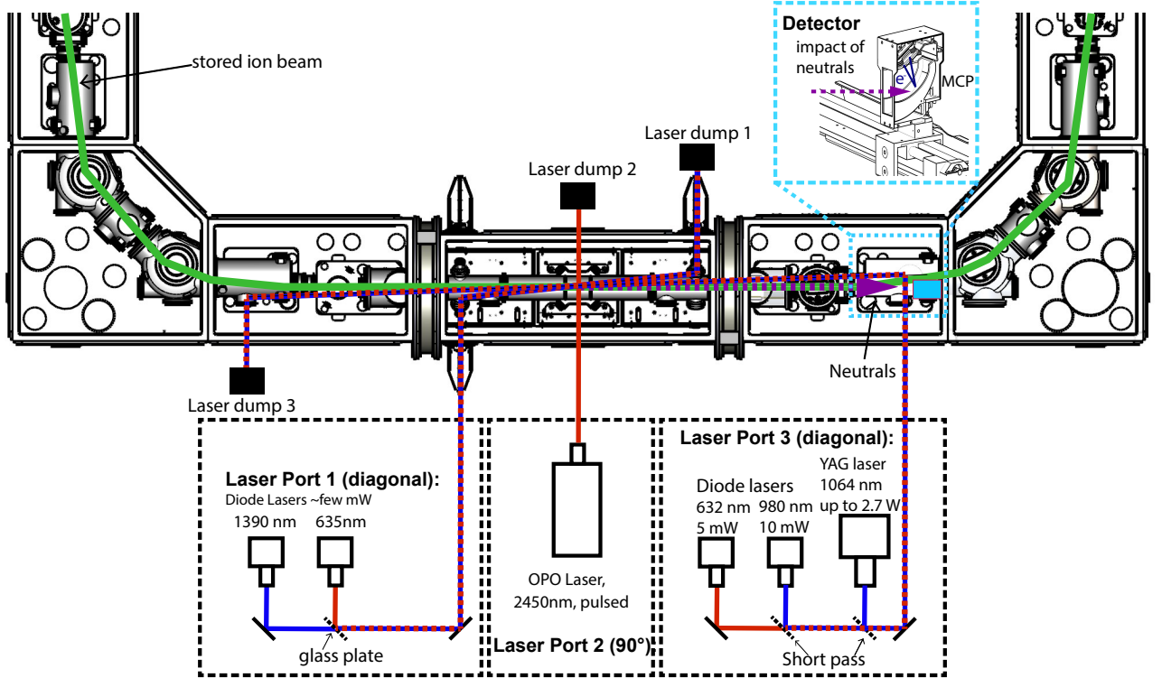
FIG. 2: Schematic of the laser interaction section at the CSR and the experimental setup (not to scale). The insets show simplified sketches of the optical setups (for the sake of simplicity not all mirrors and optical elements are shown) at the laser entry ports, and the movable single-particle detector (“Cold Movable PArticle CounTer”, COMPACT [35, 36]) that was used to detect the neutralized atoms in the present experiment.
