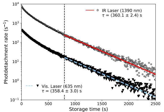
FIG. 5: Photodetachment signals for the IR laser (gray dots) and for the Vis laser (black triangles) fitted with a single exponential at storage times t > 800 s. For clarity the IR laser signal has been multiplied by a factor of 10.
