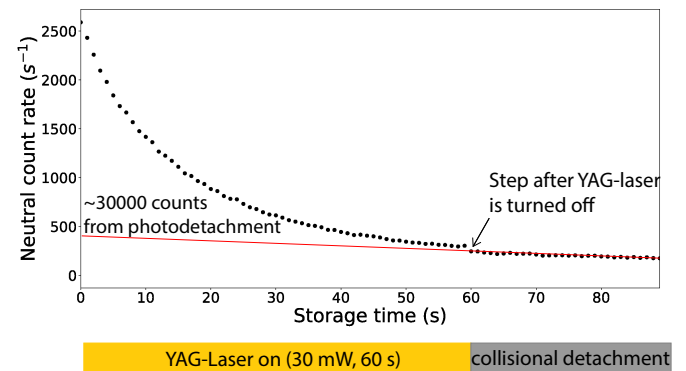
FIG. 7: Neutral count rates during a depletion run at comparatively low power. The Nd:YAG-laser was switched on for 60 s. The red curve shows a single exponential decay, which is fitted to the laser-off phase and extrapolated to shorter times. The number of counts from photodetachment is derived by integration of the events during the laser-on phase after subtraction of the extrapolated curve. We can use this value to estimate the fraction of ions in metastable states (see main text for details).
