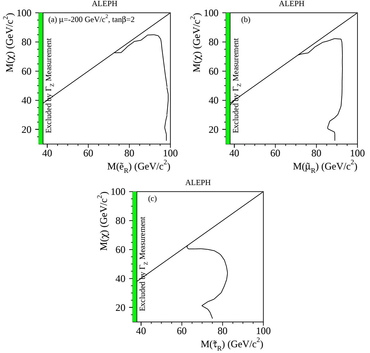
Figure 13: The 95% C.L. limits in the (m_\chi, m_{\tilde{\ell}}) plane for (a) selectrons , (b) smuons and (c) staus decaying indirectly via a dominant \tilde{U}\tilde{D}\tilde{D} operator. The selectron cross section is evaluated at \mu = -200 GeV/c 2 and \tan\beta = 2 .
