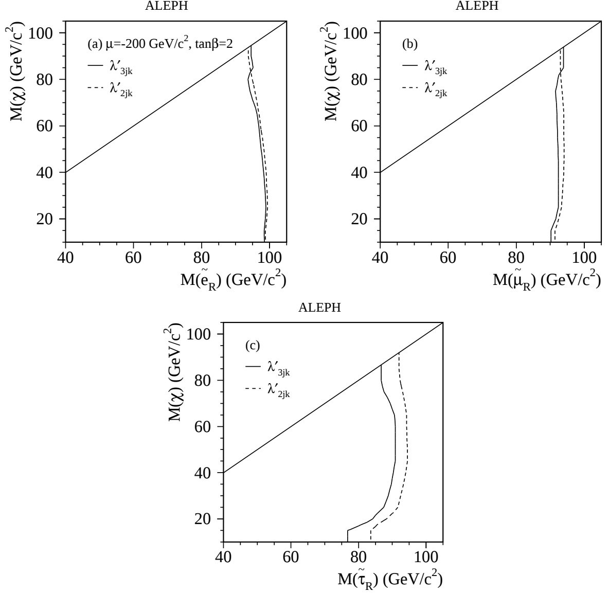
Figure 10: The 95% C.L. limits in the (m_\chi, m_{\tilde{\ell}_R}) plane for (a) selectrons, (b) smuons and (c) staus decaying indirectly via a dominant LQ\bar{D} operator. The two choices of \lambda'_{2jk} and \lambda'_{3jk} correspond to the most and least stringent exclusions, respectively. The selectron cross section is evaluated at \mu = -200 \text{ GeV}/c^2 and \tan\beta = 2 . The limit from the \Gamma_Z measurements excludes m_{\tilde{\ell}} < 38 \text{ GeV}/c^2 .
