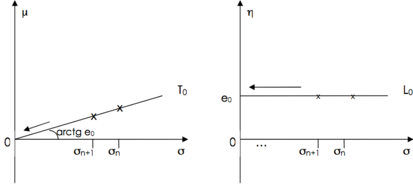
Figure 1: A same converging sequence in two parameterizations.
