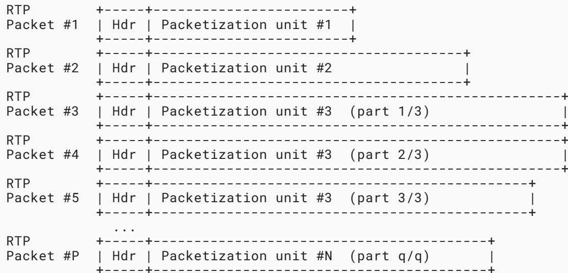
Figure 1: Example of ADU Packetization
