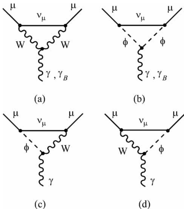
FIGURE 1. W -boson (and would-be Goldstone) contributions to a_\mu .
