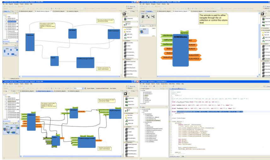
Figure 3: OpenInterface includes a visual editor called SKEMMI that can be used to design both the diagrams and the components that participate in an OpenInterface application. Diagrams can be visualized at several levels of detail and executable code can be automatically generated from them.
