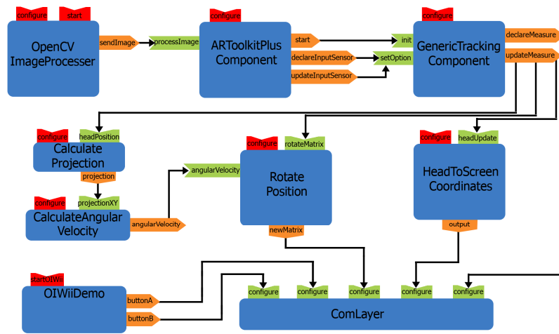
Figure 6. OpenInterface Pipeline used for prototype number 4.
