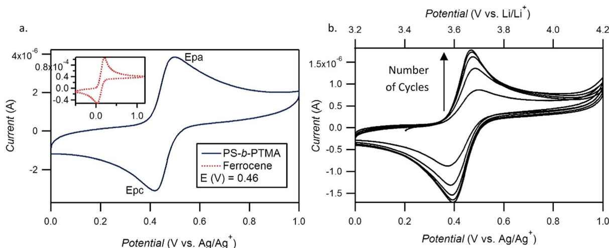
Fig. 6 Cyclic voltammogram of PTMA 79 - b -PS 502 (0.1 \text{mV s}^{-1} ; working = Pt disk (left) or ITO substrate (right); counter = Pt wire; ref. = \text{Ag}/\text{Ag}^+ (0.01 M \text{AgNO}_3 + 0.1 M \text{TBAClO}_4 ) electrolyte = 0.1 M \text{TBAClO}_4 in \text{CH}_3\text{CN} ). (a) PTMA- b -PS in solution; (b) PTMA- b -PS thin film (potential vs. \text{Li}/\text{Li}^+ calculated).
