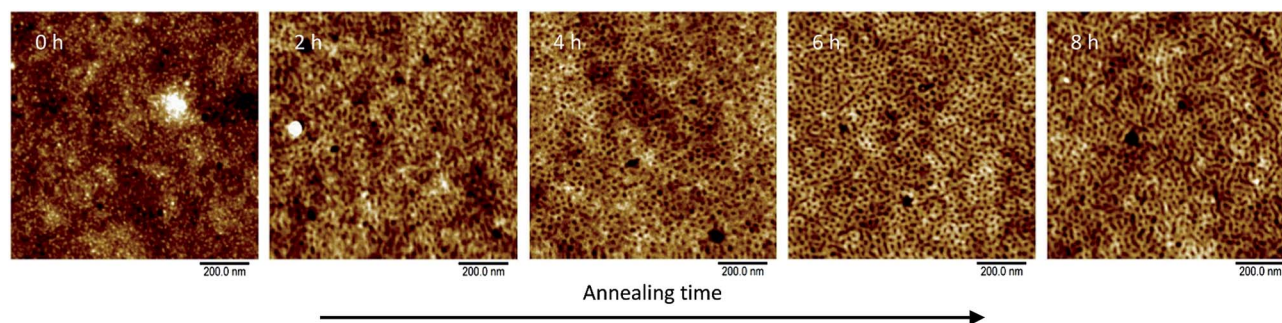
Fig. 3 AFM height images of PTMA 32 - b -PS 336 thin films after annealing with DMF (L) and DEC (M) during different times. From no solvent annealing effect (left) to a strong solvent annealing effect after 8 h (right).
