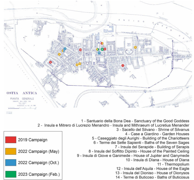
Figure 1. Map of Ostia Antica showing the different buildings studied in 2019 (red), May 2022 (yellow), October 2022 (blue), and 2023 (green).
