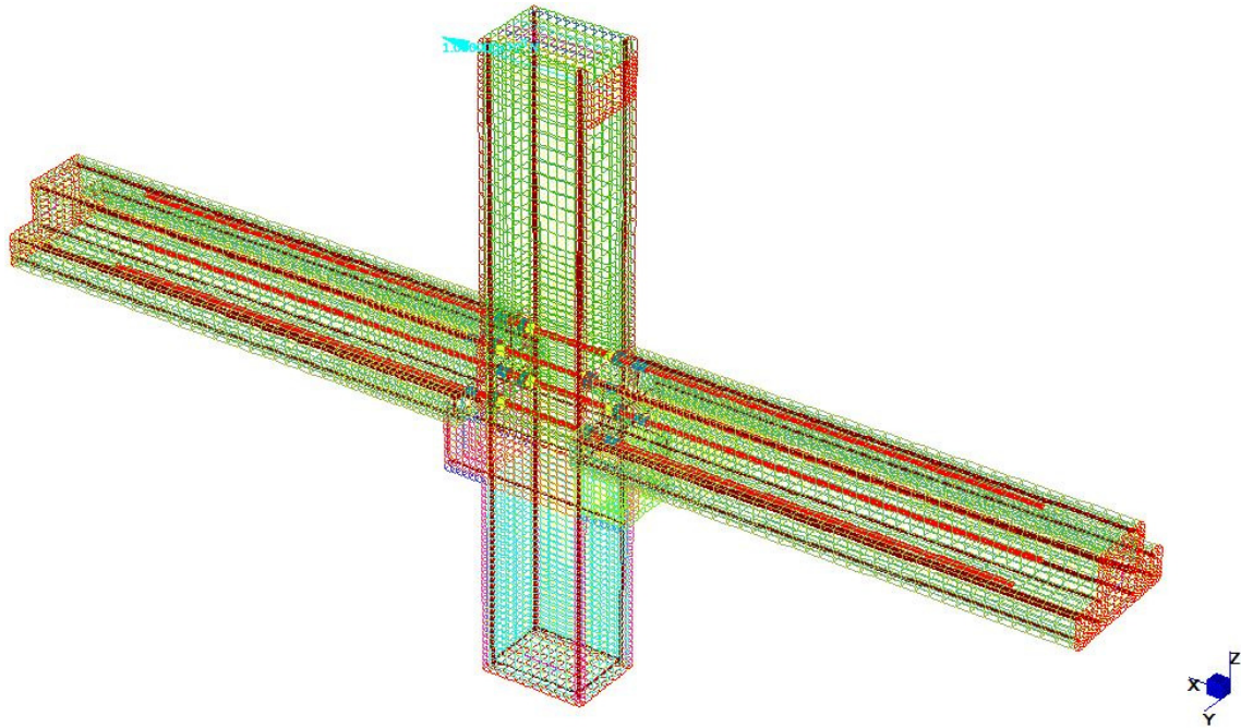
Fig.4. Application of the BS-Italy connection system, meso-level FE model.
