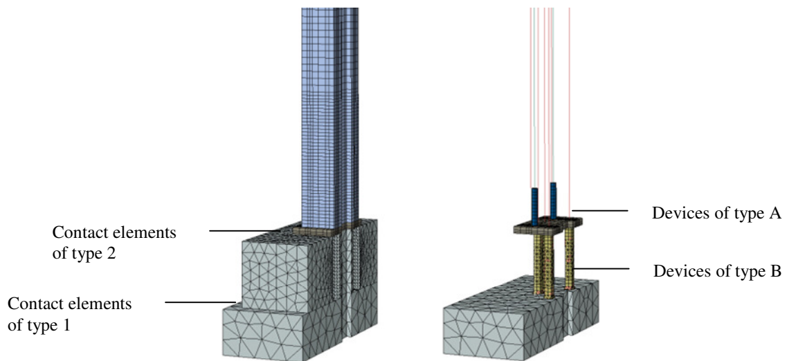
Fig.8. Location of elements of the continuity system.
