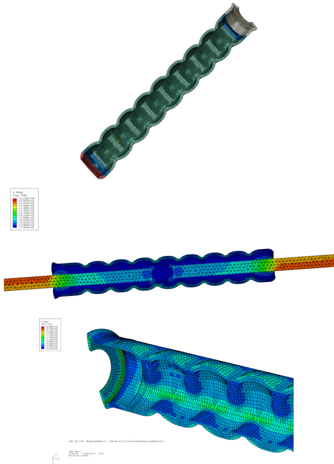
Fig. 3. BS-Italy connection system, micro-level FE model.
