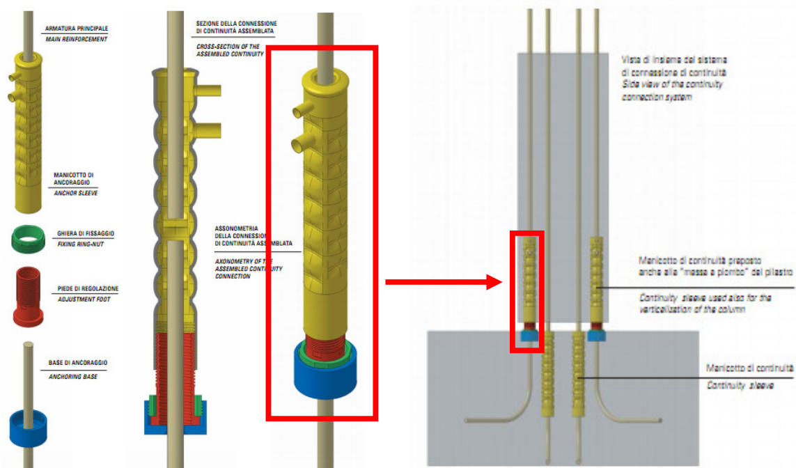
Fig.1. Concept of the BS-Italy connection system.
