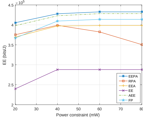
Figure 7.2: EE performances versus power constraints. d_1 = d_2 = 15 m.
