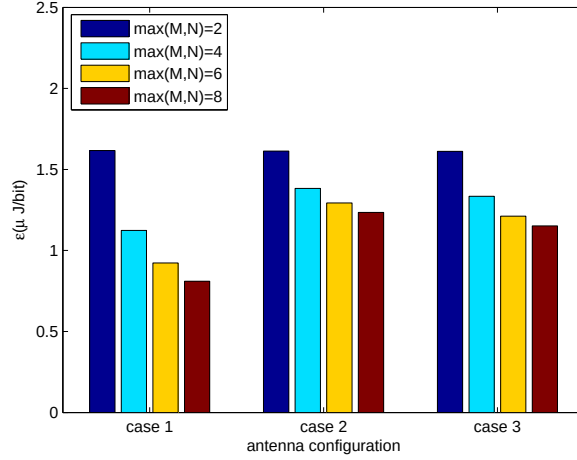
Figure 3.4: Power consumption and EE comparison for different antenna configurations with d=50\text{m} and K=32 .
