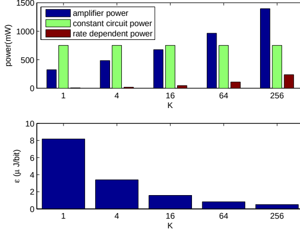
Figure 3.2: Power consumption and EE comparison for different K with M = N = 4 and d=50 m.
