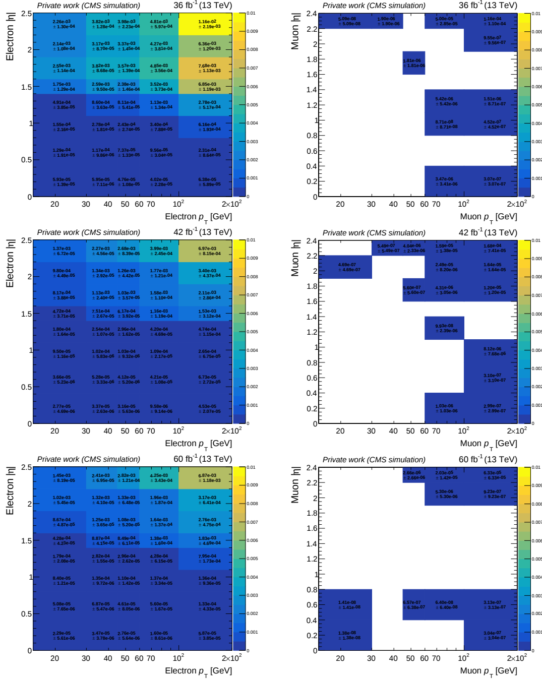
Figure 3.8: The charge misID rate of electron (left) and muon (right) measured in t\bar{t} , t\bar{t}W , and WZ simulation samples by comparing the reconstructed charge to the generated charge of the leptons. The figures are arranged in descending order: 2016 (top), 2017 (middle), and 2018 (bottom) simulations.
