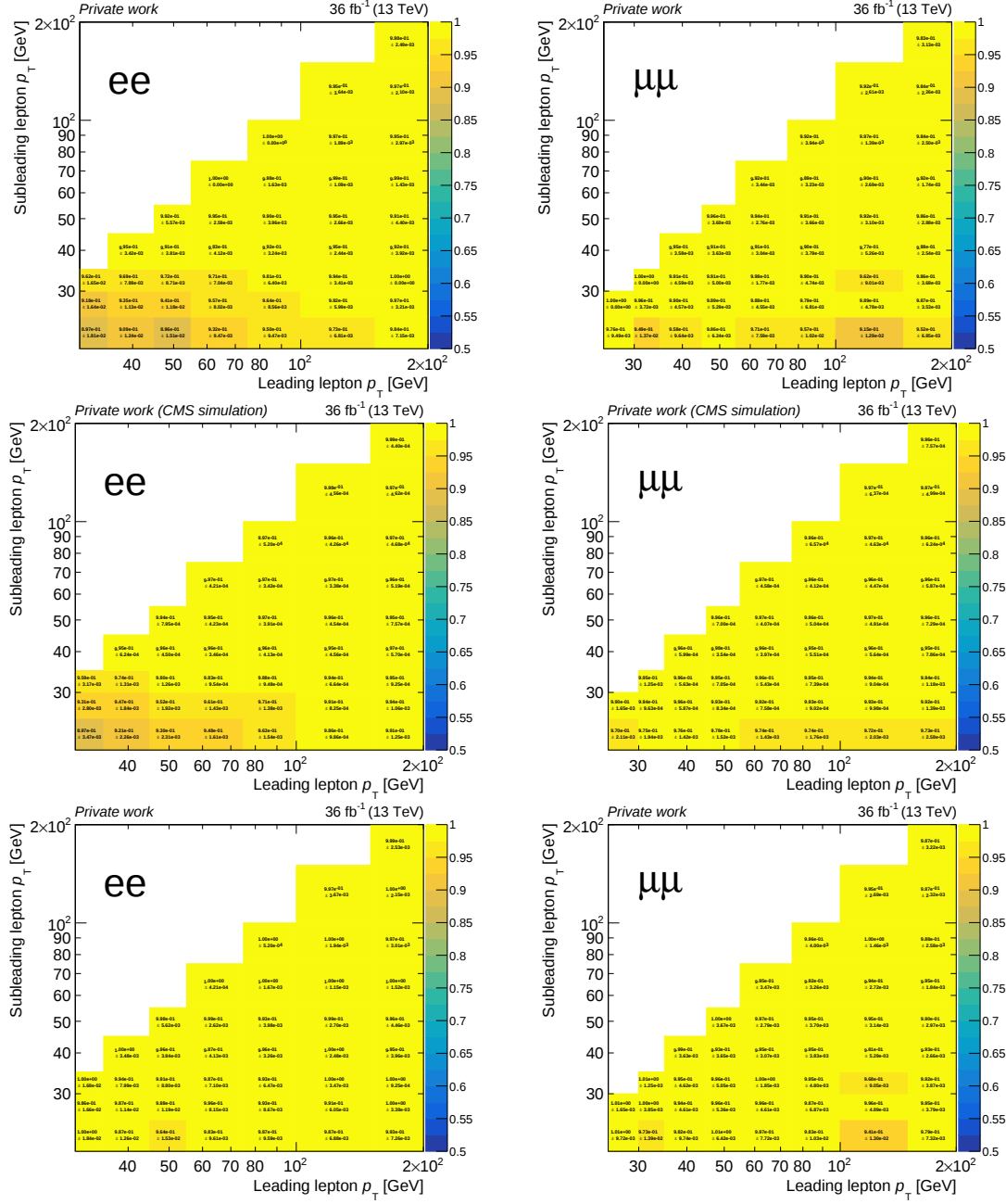
Figure 3.1: Trigger efficiencies measured in 2016 JetMET+JetHT data sets (top row) and t\bar{t} simulations (middle row), categorised by di-electron (left column) and di-muon (right column) channels. The associated scale factors for these efficiencies are presented in the bottom row.
