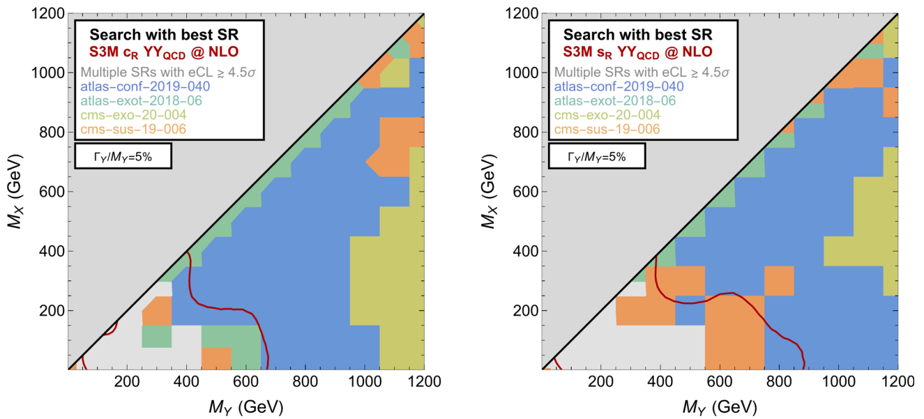
Fig. 6 Search including the most sensitive signal region for the new physics signal emerging from the YY_{\text{QCD}} processes at NLO, for the S3M\_cR (left) and S3M\_sR (right) models with a fixed width-to-mass ratio. The 95% CL exclusion limit is also reported
