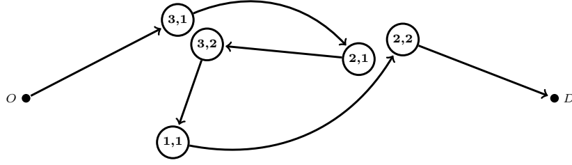
Figure 3: Route given in Figure 1 represented in G^V .
