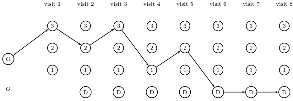
Figure 6: Example of a path in the extended network for a maximum of eight visits and three locations.
