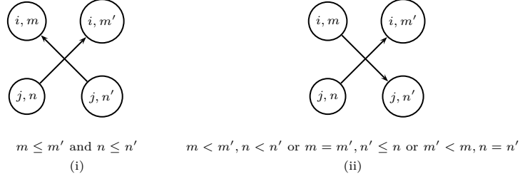
Figure 4: Incompatible arc pairs.
