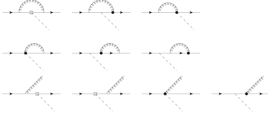
FIG. 2. Virtual and real corrections for t \rightarrow uh . The squares represent the contribution from O_{u\phi} , while the black dots represent the contribution from O_{uG} .
