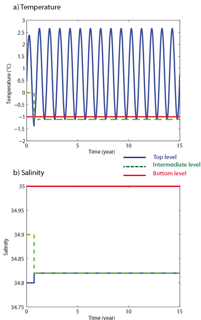
Fig. 7. (a) Temperature (°C) and (b) salinity in an experiment performed with the three-level model initialized from a weakly stratified state. The value of the top level is in blue, the intermediate level in green and the bottom one is in red. In this configuration, the top two levels interact every winter and no ice is formed.
