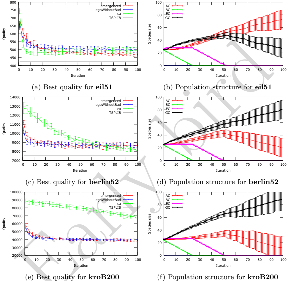
Figure 2. Instances eil51 , berlin52 , and kroB200 , migration from worst to best species with 2% decrease in quality
