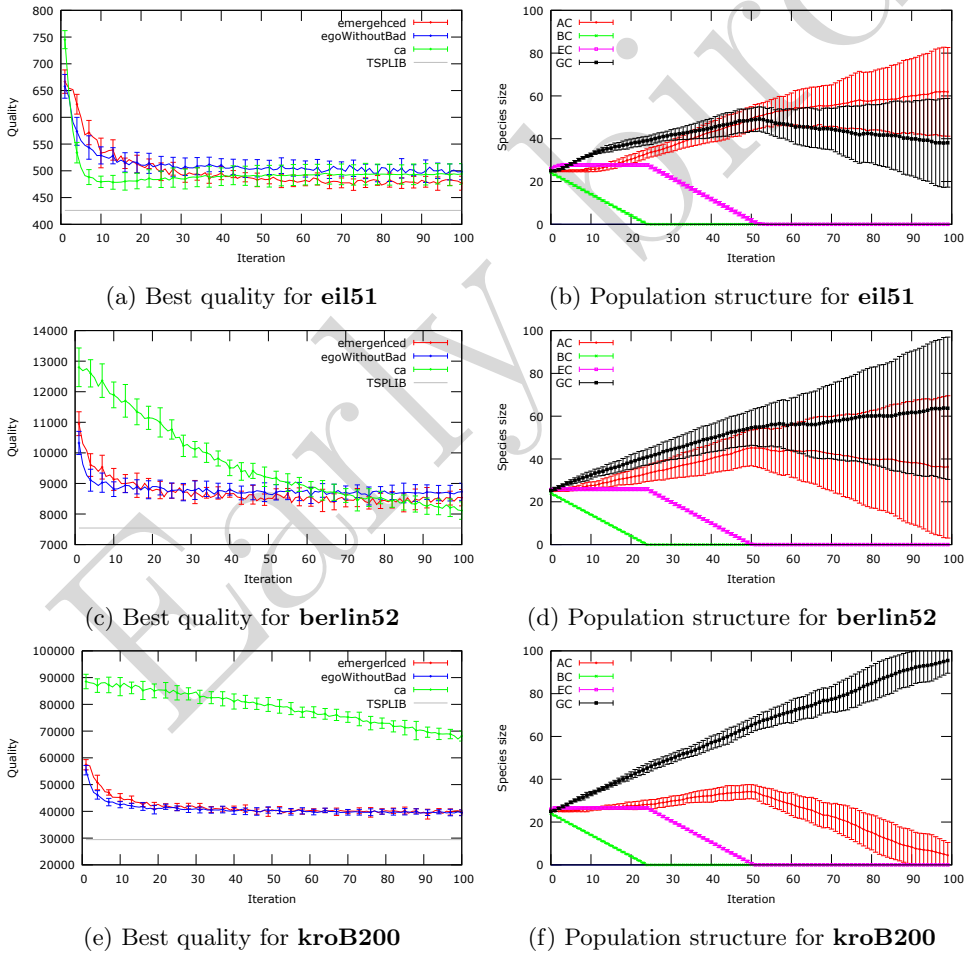
Figure 3. Instances eil51 , berlin52 , and kroB200 , stepwise migration of one ant assuming quality decrease of 2%
