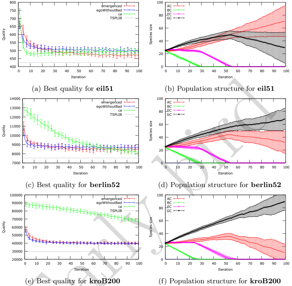
Figure 6. Instances eil51 , berlin52 , and kroB200 , stochastic migration
