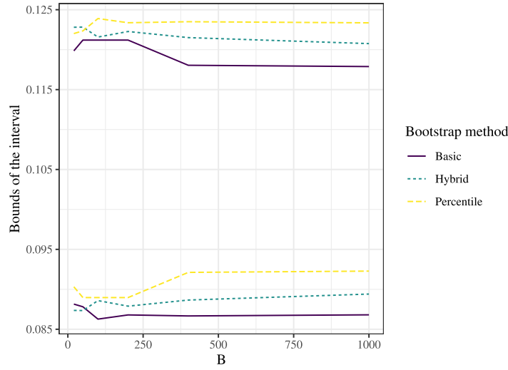
FIG 5. Evolution of the confidence interval for G_{iY,X} for the SCAD-FABS ( n_{fwd} = 20 ) on the Griliches data.
