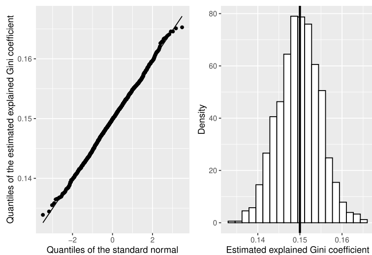
FIG 8. Asymptotic Normality of \widehat{Gti}_{Y,X} obtained with the PLR-SCAD on Setup 1, samples of size 1000.
