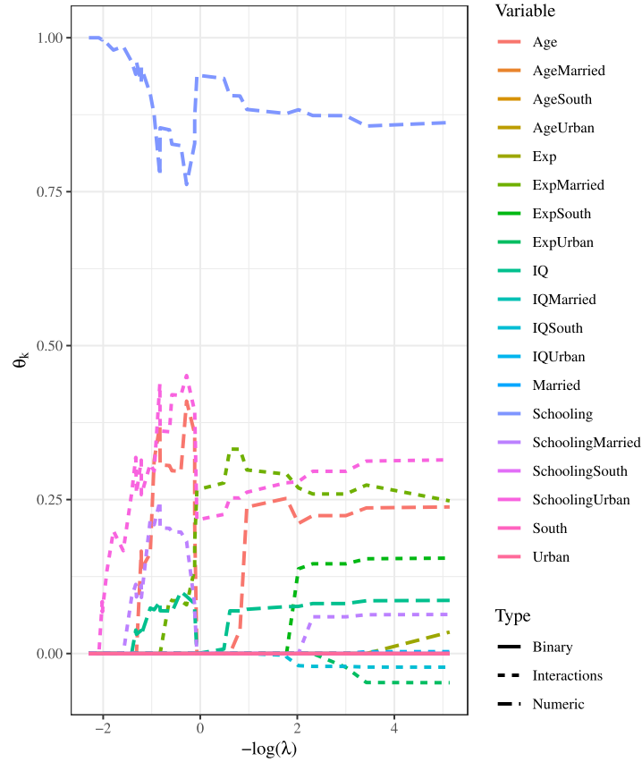
FIG 3. Trace plot of the SCAD-FABS ( n_{fwd} = 20 ) on the Griliches data.
