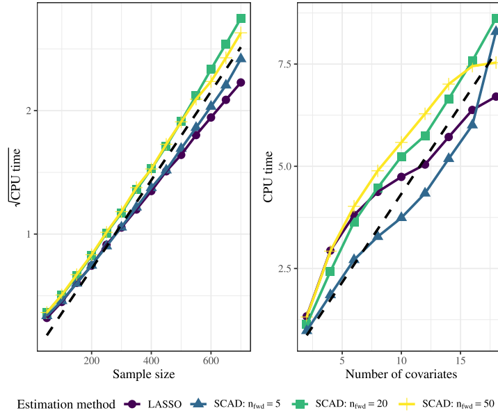
FIG 6. Evolution of the run time as a function of n and p on the Griliches data.
