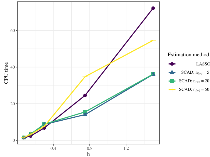
FIG 7. Evolution of the CPU time in function of h on the Griliches data.
