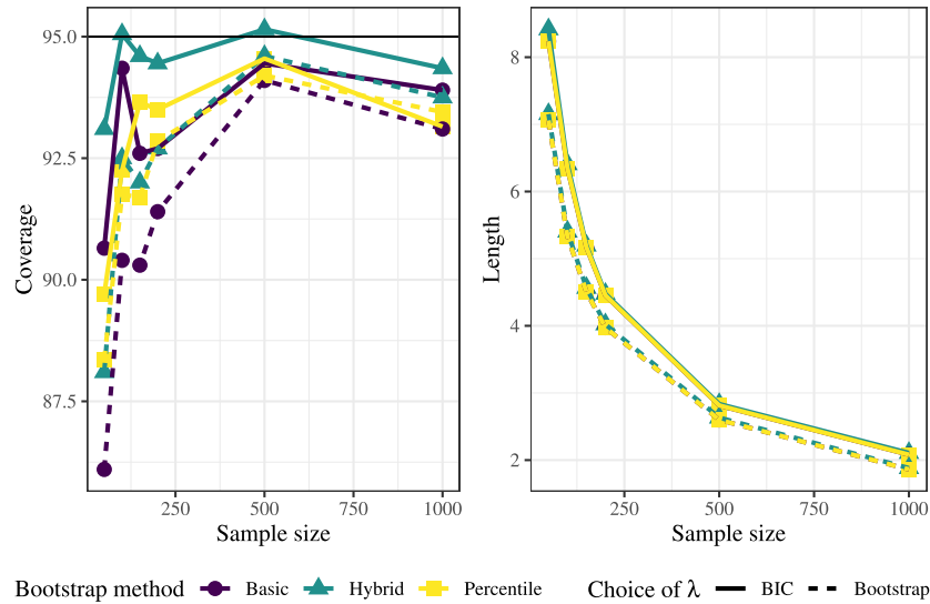
FIG 2. Coverages and Lengths of confidence intervals for G_{iY,X} on Setup 1.
