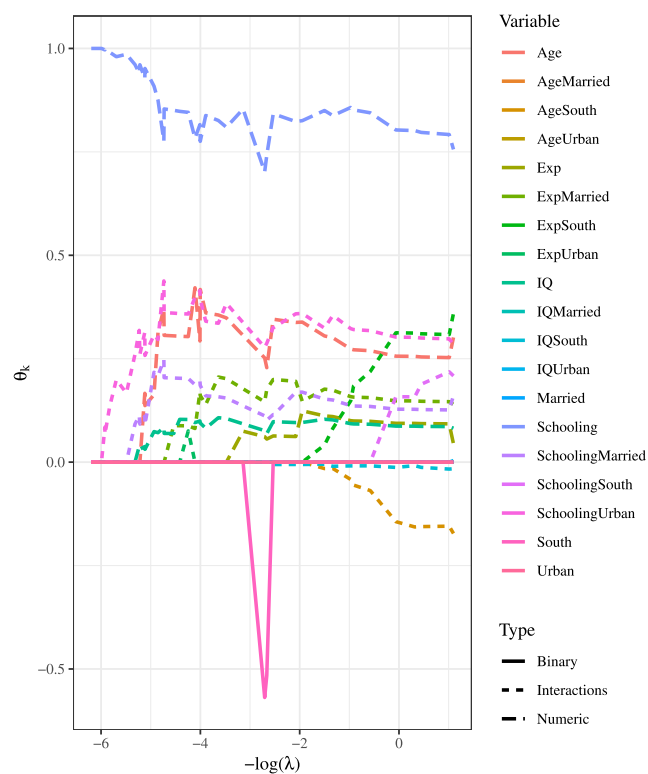
FIG 9. Trace plot of the FABS on the Griliches data.
