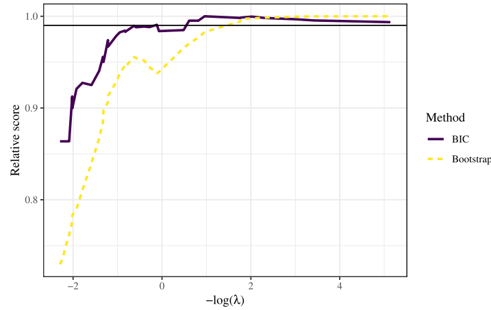
FIG 4. Evolution of the BIC and OOB-scores for the SCAD-FABS ( n_{\text{fwd}} = 20 ) on the Griliches data.
