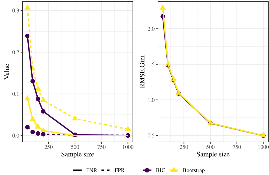
FIG 1. Consistency of the PLR-SCAD on Setup 1.
