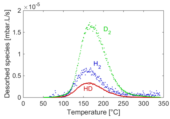
Figure 1 – Different contributions of the thermal desorption analysis of a sample containing H and D.
