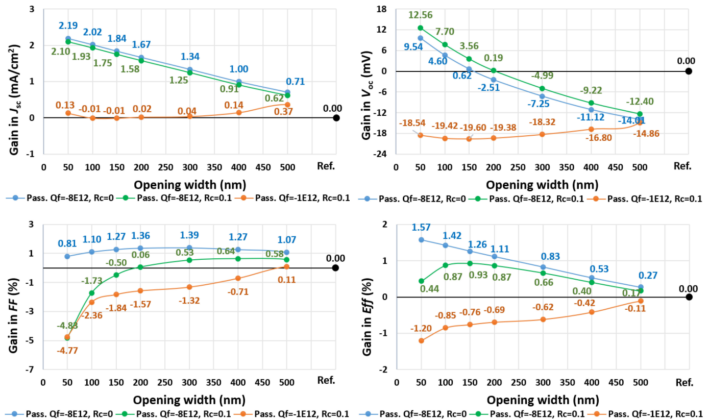
Fig. 6. Gains on absolute values of PV-parameters for passivated UT-CIGS cells for different opening widths at fixed pitch of 0.5 \mu\text{m} with and without R_c and for two Q_f densities: Q_f = -8 \times 10^{12} \text{ cm}^{-2} with R_c = 0 \Omega\text{-cm}^2 (blue curves), Q_f = -8 \times 10^{12} \text{ cm}^{-2} with R_c = 0.1 \Omega\text{-cm}^2 (green curves), and Q_f = -1 \times 10^{12} \text{ cm}^{-2} with R_c = 0.1 \Omega\text{-cm}^2 (red curves). The results show several dependencies highlighting that several parameters enter into play when defining the best pattern of the rear passivation.
