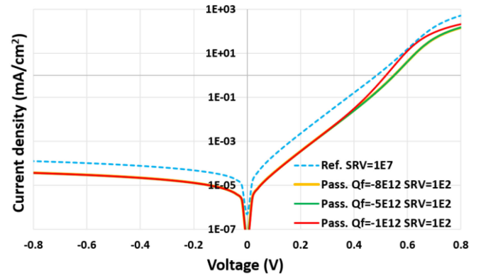
Fig. 5. Simulated J - V curves in the dark for reference cells (blue dashes) with an SRV of 1 \times 10^7 cm.s -1 and passivated cells with an SRV of 1 \times 10^2 cm/s with three different Q_f values of -8 \times 10^{12} cm -2 (yellow lines), -5 \times 10^{12} cm -2 (green lines), and -1 \times 10^{12} cm -2 (red lines). The yellow line is overlapped with the green one. Simulation reproduces the trends of the experiment showing the effect of the Q_f density on the electrical performances of the cell.
