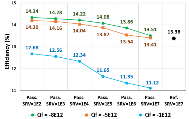
Fig. 4. Efficiency of reference cell with \text{SRV} = 1 \times 10^7 cm/s and passivated cells with different SRV values from 1 \times 10^2 to 1 \times 10^7 cm/s and different Q_f densities ( -8 \times 10^{12} cm -2 , -5 \times 10^{12} cm -2 , -1 \times 10^{12} cm -2 ). The passivated cells with the highest Q_f density show better efficiency above the reference for each SRV value indicating the importance of the negative oxide charges to improve the cell performances.
