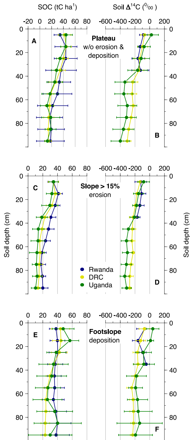
Fig. 6. Mean \Delta^{14}\text{C} data for the three different sites in Rwanda, DRC, and Uganda calculated from the sites at the plateaus (no erosion or deposition), sites with slopes > 15\% , and the footslopes. Number of samples per site and depths between 5 and 13; Soil \Delta^{14}\text{C} data for Rwanda are only given to a depth of 0.4 m as fossil geogenic carbon in deeper layers of some plateaus in Rwanda give misleading values. Error bars give 95 %-confidence intervals of the mean.
