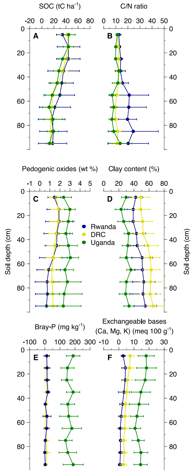
Fig. 3. Mean soil organic carbon stocks as well as important other properties at plateau positions without erosion in the different test regions in Rwanda (n = 6), Uganda (n = 5) and DRC (n = 8). Error bars give 95 %-confidence intervals of the mean (data taken from S. Doetterl et al., 2021; Reichenbach et al., 2023).
