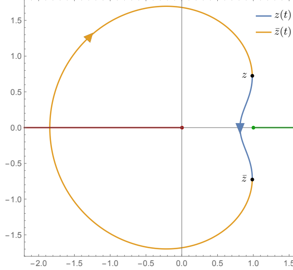
Figure 1: Paths in the complex plane for the analytic continuation of the variables z and \bar{z} to the physical region where partons 1 and 2 are incoming.
