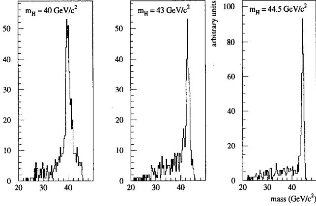
Fig. 3. Mass distributions obtained after constrained fitting of simulated events for three Higgs boson masses. Full widths at half maximum are respectively 1.7 (1.1) (0.8) \text{GeV}/c^2 at m_H = 40 (43) (44.5) \text{GeV}/c^2
