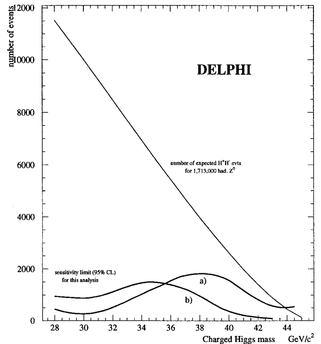
Fig. 8. Limit of sensitivity of the hadronic analysis (two methods), compared with the total number of expected signal events, showing clearly the exclusion interval from 28 to 43.5 GeV/c 2 . Curve a) is obtained by a direct comparison of data versus background and curve b) by a fit to data + \alpha \times signal
