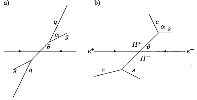
Fig. 4. Schematic diagrams of a) background, b) signal events
