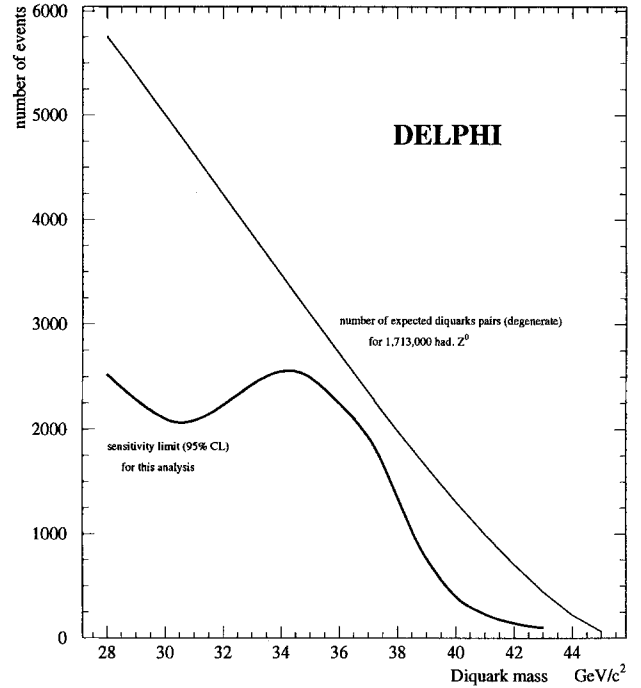
Fig. 10. Limit of sensitivity of the diquark analysis, compared with the total number of expected signal events, showing clearly the exclusion interval from 28 to 43 \text{GeV}/c^2
