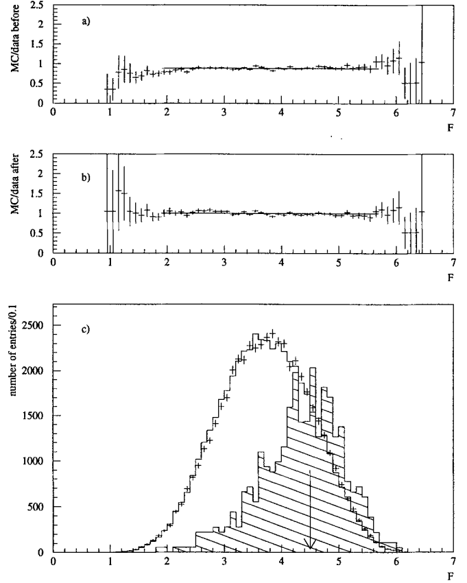
Fig. 6. Above, MC/data ratio as a function of F (see equation (2) for definition), a) before and b) after y_{cut} fixing. The fits of this ratio to a constant value give the following results : a) 0.885 and \chi^2 = 44.3 for 37 degrees of freedom and b) 0.999 and \chi^2 = 43.2 for the same number of degrees of freedom. Below (c), distribution of the variable F for q\bar{q} simulation (histogram), DELPHI data (crosses) and for a 43 \text{ GeV}/c^2 charged Higgs boson (hatched histogram, not to scale). The cut at 4.5 is indicated by the vertical arrow
