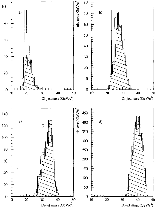
Fig. 11. Comparison between di-jet mass spectra for simulation (shaded histogram) and data (crosses), together with the expected diquark signals (unshaded) for different diquark masses : a) 17.5 GeV/c 2 non-degenerate, b) 23 GeV/c 2 non-degenerate, c) 29 GeV/c 2 degenerate and d) 36.5 GeV/c 2 degenerate diquarks
