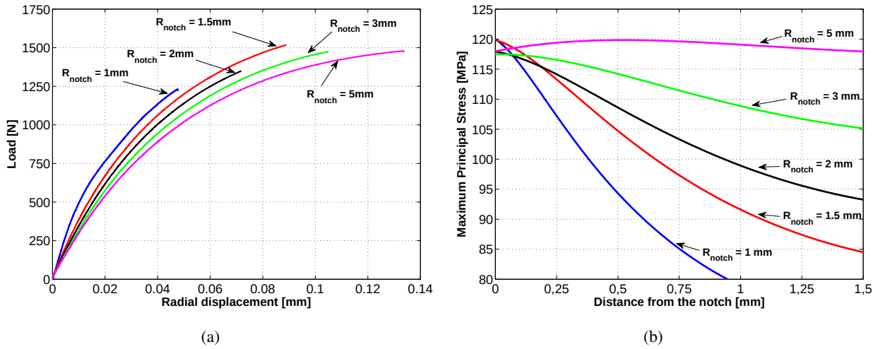
Figure 6: a) Reference load-displacement curves of the tensile tests on notched specimens; b) variation of the maximum principal stress as a function of the distance to the notch root right at failure, computed by FE analyses.
