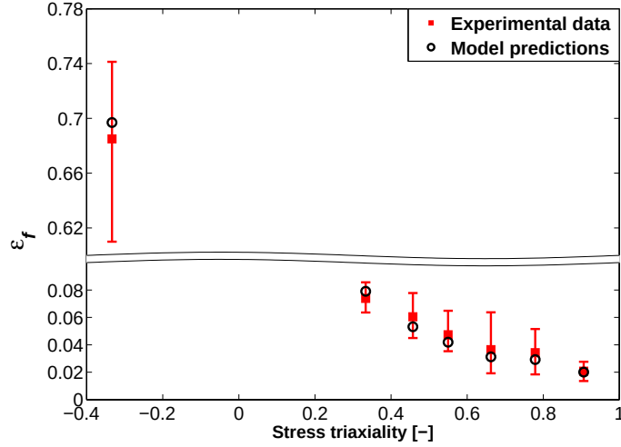
Figure 9: Variation of the experimental and predicted equivalent fracture strain \varepsilon_f as a function of the mean stress triaxiality in all the tested specimens (except compression with barreling), involving the error bars corresponding to the experimental data dispersion ; the dots represent the predicted \varepsilon_f corresponding to a local MPS = 300MPa and an aspect ratio A_r = 0.27 .
