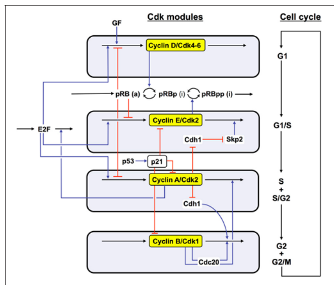
FIGURE 1 | Detailed model for the Cdk network driving the mammalian cell cycle. The model incorporates four modules centered on the main cyclin/Cdk complexes: cyclin D/Cdk4–6, cyclin E/Cdk2, cyclin A/Cdk2, and cyclin B/Cdk1. Also considered are the effect of the growth factor GF and the roles of pRB and E2F which exert antagonistic controls on cell cycle progression. Cyclin D/Cdk4–6 and cyclin E/Cdk2 control progression in G1 and the G1/S transition by phosphorylating, and thereby inhibiting, pRB. The rise in cyclin A/Cdk2 permits progression in S and G2, while the peak of cyclin B/Cdk1 brings about the G2/M transition. The active, unphosphorylated form of pRB inhibits E2F, which promotes cell cycle progression by inducing the synthesis of cyclins D, E, and A. The protein Cdh1, inhibited by cyclin A/Cdk2, promotes the degradation of cyclin B, and inhibits Skp2, which promotes the degradation of cyclin E; activation of cyclin A/Cdk2 thus leads to the activation of cyclin B/Cdk1 and to the inhibition of cyclin E/Cdk2. The protein Cdc20, activated by cyclin B/Cdk1, promotes the degradation of cyclin A and cyclin B, which leads to the decrease in cyclin A/Cdk2 and cyclin B/Cdk1. For the sake of clarity, not all regulations considered in the model are shown in this scheme—see supporting information in Gérard and Goldbeter (2009) for more detailed schemes of the model for the Cdk network. The combined effects of the regulatory interactions between the four Cdk modules give rise to sustained Cdk oscillations (see Figure 2) that allow the cell to progress in a repetitive, oscillatory manner along the successive phases of the cell cycle depicted on the right part of the figure (Gérard and Goldbeter, 2009).
