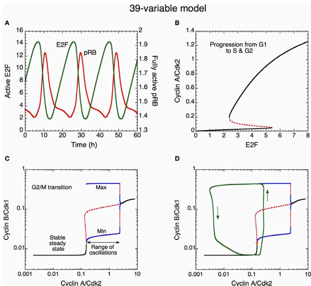
FIGURE 10 | Mechanism of oscillations in the Cdk network. (A) The curves show the time evolution of the active, unphosphorylated, forms of E2F (in green) and pRB (in red) which oscillate in antiphase. (B) Bifurcation diagram showing the steady-state level of cyclin A/Cdk2 as a function of E2F, considered as a parameter. Two stable steady states coexist in the domain of bistability. The sharp increase in cyclin A/Cdk2 above a critical level of E2F favors progression from the cell cycle phase G1 to S and G2. (C) Bifurcation diagram showing the steady-state level of cyclin B/Cdk1 as a function of cyclin A/Cdk2, considered as a parameter. A domain of sustained oscillations exists above a critical level of cyclin A/Cdk2; the upper and lower blue curves denote the maximum and minimum of cyclin B/Cdk1 oscillations as a function of cyclin A/Cdk2. The rise in the level of cyclin A/Cdk2 pushes transiently the system into the domain of sustained oscillations, which permits the activation of cyclin B/Cdk1 at the G2/M transition. The rise in cyclin B/Cdk1 leads to the activation of the protein Cdc20, which promotes the degradation of cyclins A and B; this creates a negative feedback loop in the activation of cyclin A/Cdk2 and cyclin B/Cdk1. The subsequent decrease
