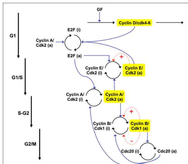
FIGURE 12 | Scheme of the extended skeleton model for the mammalian cell cycle (Gérard et al., 2012). The model contains the four main cyclin/Cdk complexes, the transcription factor E2F, and the protein Cdc20. Growth factor (GF) induces entry in the G1 phase of the cell cycle by promoting the synthesis of cyclin D/Cdk4–6. The latter complex allows the activation of E2F, which elicits the synthesis of cyclin E/Cdk2, at the G1/S transition, and cyclin A/Cdk2, during the S phase of DNA replication. During G2, cyclin A/Cdk2 also activates the synthesis of cyclin B/Cdk1, which elicits the peak of activity of cyclin B/Cdk1 at the G2/M transition. During mitosis, cyclin B/Cdk1 activates by phosphorylation the protein Cdc20. This creates a negative feedback loop in the activity of cyclin A/Cdk2 and cyclin B/Cdk1 by promoting the degradation of these complexes. The regulations exerted by Cdc20 allow the cell to complete mitosis, and to start a new cycle if GF is present in sufficient amount. In this version of the model, we consider that the total concentrations of cyclin E/Cdk2, cyclin A/Cdk2, and cyclin B/Cdk1 remain constant. These complexes can vary between an active (a) and an inactive (i) form. Moreover, positive feedback (PF) loops can be added in the regulation of cyclin E/Cdk2 and cyclin B/Cdk1, which control the G1/S and G2/M transitions (dashed arrows in red). These PF loops are due to the mutual activation between Cdk2, Cdk1, and their phosphatase Cdc25 and to the mutual inhibition between Cdk1 and the kinase Wee1.
