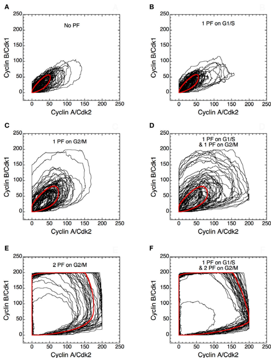
FIGURE 15 | Positive feedback loops increase the robustness of limit cycle oscillations in the Cdk network. Projection of the stochastic limit cycle (black curve) and the corresponding deterministic limit cycle (red curve) in the cyclin A/Cdk2 vs. cyclin B/Cdk1 plane. Numerical simulations were performed in the extended version of the skeleton model for the mammalian cell cycle (Gérard et al., 2012) (A) in the absence of PF loop ( b_1 = 0 , b_2 = 0 , K_{ib} = 1000 \mu\text{M} ), or in the presence of (B) one PF on G1/S via Cdc25 ( b_1 = 1 , b_2 = 0 , K_{ib} = 1000 \mu\text{M} ), (C) one
