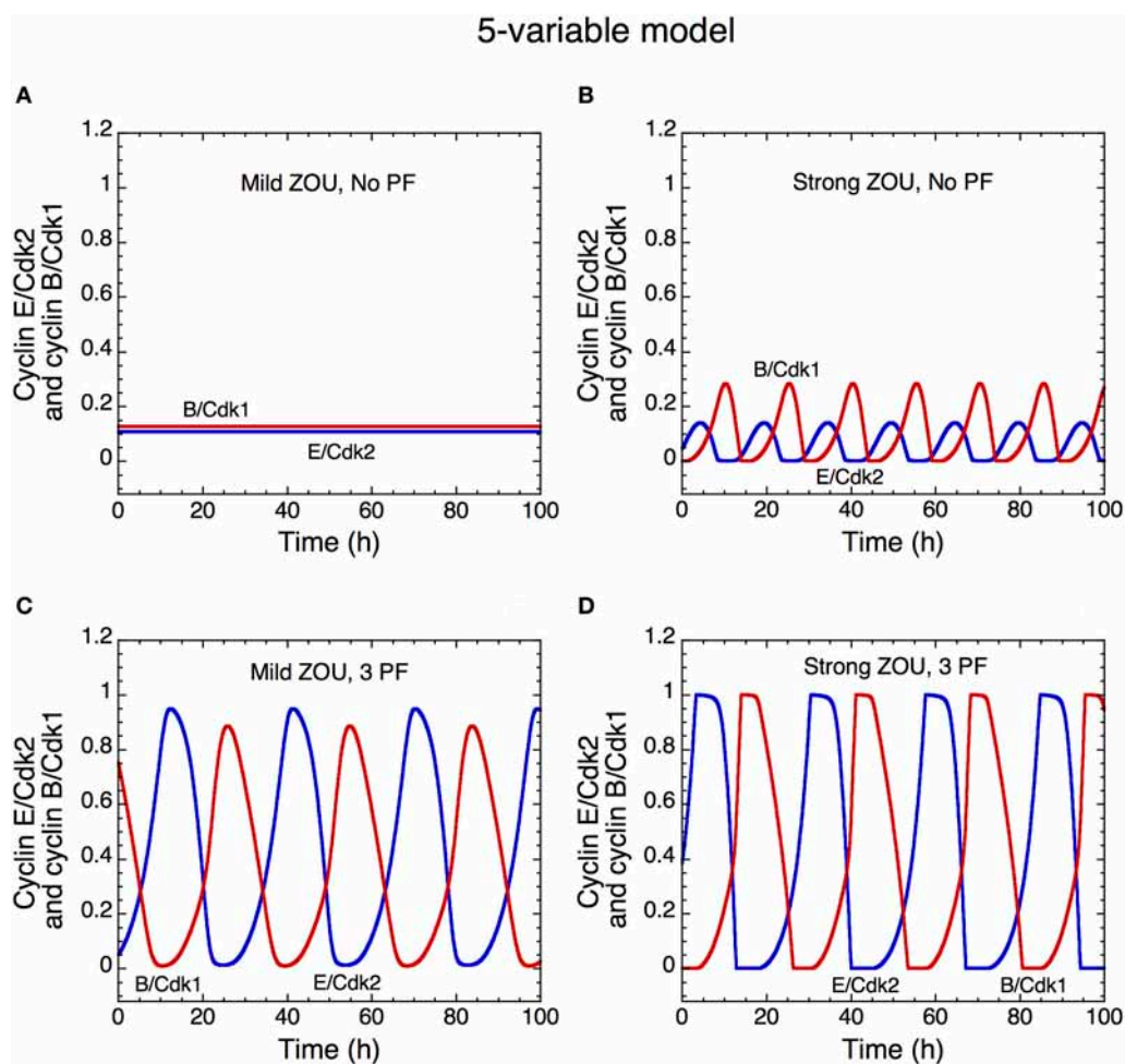
FIGURE 13 | Oscillatory dynamics of the skeleton model for the Cdk network driving the mammalian cell cycle: role of zero-order ultrasensitivity (ZOU) and positive feedback. The curves show the time evolution of cyclin E/Cdk2 (in blue) and cyclin B/Cdk1 (in red) in the presence of mild ultrasensitivity ( K = 0.1 \mu\text{M} in A and C ) or strong ultrasensitivity ( K = 0.005 \mu\text{M} in B and D ), and in the absence of any PF loop ( b_1 = 0 , b_2 = 0 , K_{ib} = 1000 \mu\text{M} in A,B ) or presence ( b_1 = 1 , b_2 = 1 , K_{ib} = 0.5 \mu\text{M} in C,D ) of three PF loops. The presence of PF loops as well as the presence of strong ultrasensitivity enhance
