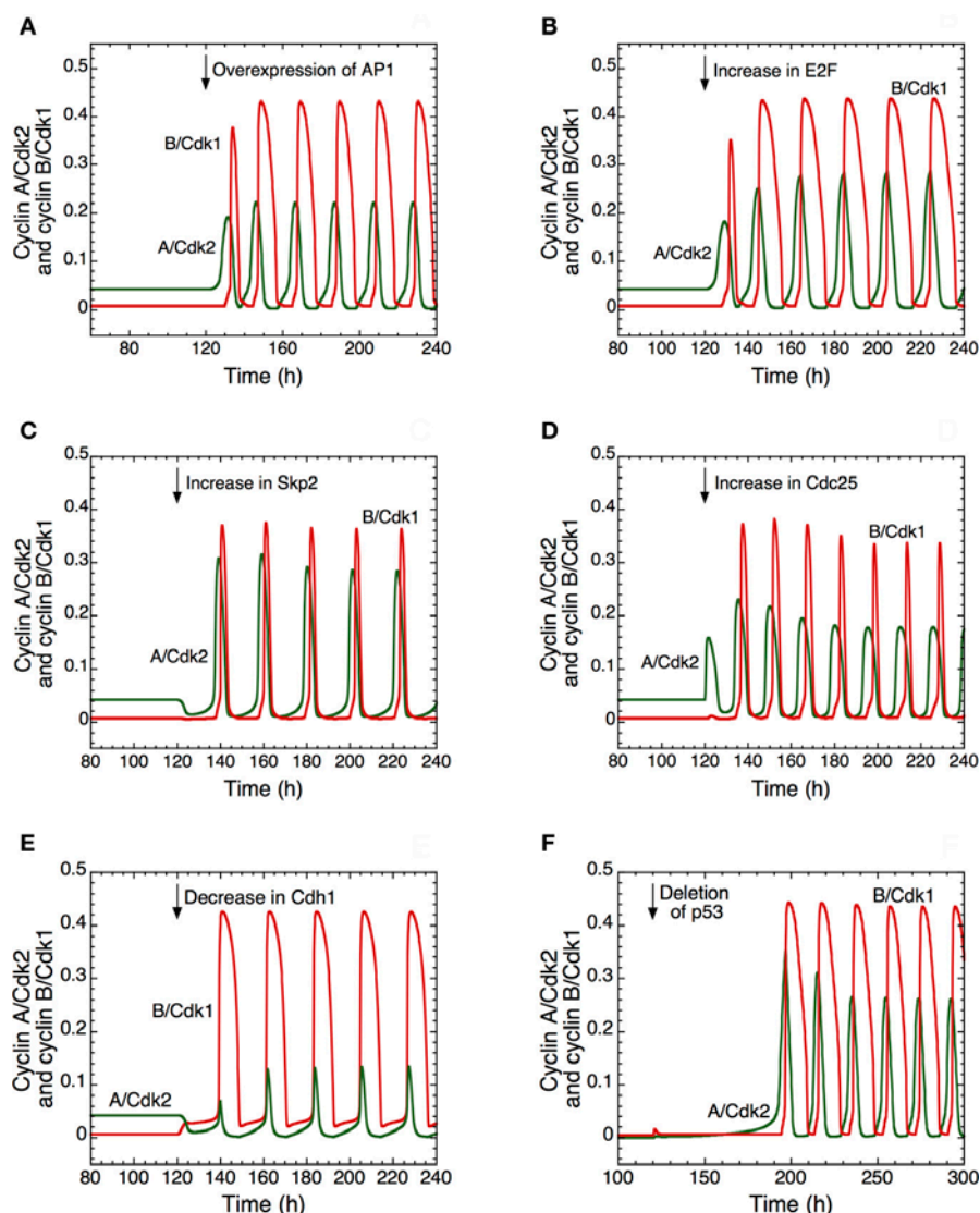
FIGURE 4 | Multiple ways to induce the passage from cellular quiescence to cell proliferation in the detailed model for the mammalian cell cycle. The switch to sustained oscillations of cyclin A/Cdk2 (in green) and cyclin B/Cdk1 (in red) is shown following the overexpression of AP1 ( A ), E2F ( B ), Skp2 ( C ), or Cdc25 ( D ), or the decrease of Cdh1 ( E ) or p53, via a decrease in p21 ( F ). In each case, from t = 120 h, the Cdk network passes from a stable steady state, corresponding to cellular quiescence, to an oscillatory regime corresponding to cell proliferation. From t = 120 h, the rate of synthesis of AP1, v_{\text{ap1}} , passes from 1 to 2 \mu\text{Mh}^{-1} in ( A ); the rate of synthesis of E2F, v_{\text{e2f}} , passes from 0.15 to 0.5 \mu\text{Mh}^{-1} in ( B ); the rate of synthesis of Skp2, v_{\text{skp2}} , passes from 0.15 to 0.5 \mu\text{Mh}^{-1} in ( C ); the rate of
