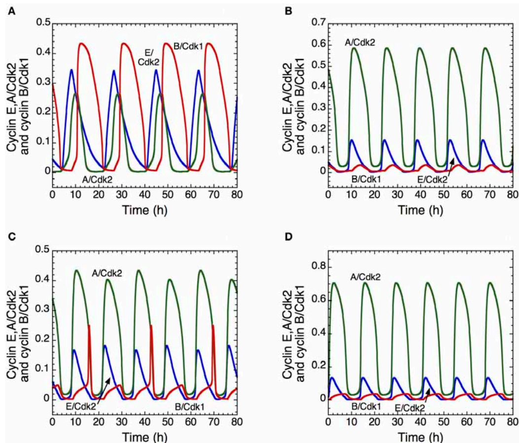
FIGURE 7 | Endoreplication or tetraploidy in the detailed model for the mammalian cell cycle. The curves show the time evolution of cyclin E/Cdk2 (in blue), cyclin A/Cdk2 (in green) and cyclin B/Cdk1 (in red) corresponding to the “classical” mitotic cell cycle in (A), to endoreplication cycles in (B) and (D); and to tetraploidy in (C). In (B), the rate of inhibition of Cdh1, V_{2cdh1} ,
