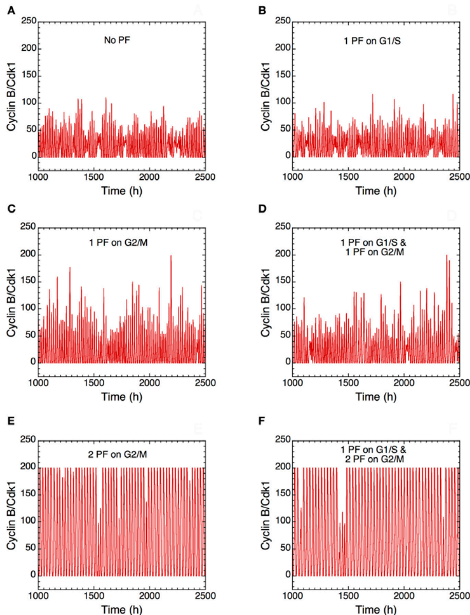
FIGURE 14 | Positive feedback loops increase the robustness of Cdk oscillations with respect to molecular noise. The long-term time evolution of cyclin B/Cdk1 is shown in the extended version of the skeleton model for the mammalian cell cycle (Gérard et al., 2012) (A) in the absence of PF loop ( b_1 = 0 , b_2 = 0 , K_{ib} = 1000 \mu\text{M} ) or in the presence of (B) one PF on G1/S via Cdc25 ( b_1 = 1 , b_2 = 0 , K_{ib} = 1000 \mu\text{M} ), (C) one PF on G2/M via Cdc25 ( b_1 = 0 , b_2 = 1 , K_{ib} = 1000 \mu\text{M} ), (D) one PF on G1/S and one PF on G2/M via Cdc25 ( b_1 = 1 , b_2 = 1 , K_{ib} = 1000 \mu\text{M} ), (E) two PF on G2/M via Cdc25 and
