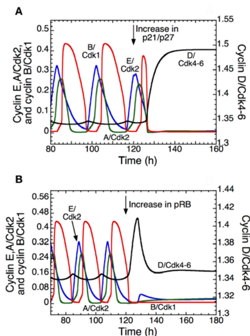
FIGURE 5 | Arresting the mammalian cell cycle in the G1 phase. The curves show the time evolution of cyclin D/Cdk4–6 (in black), cyclin E/Cdk2 (in blue), cyclin A/Cdk2 (in green), and cyclin B/Cdk1 (in red) in the detailed model for the Cdk network. In t = 120 h, the transition from a sustained oscillatory regime of the Cdk network, corresponding to cell proliferation, to a stable steady state corresponding to cell cycle arrest follows the overexpression of p21–p27 when v_{sp27} passes from 0.8 to 5 \mu\text{Mh}^{-1} (A), or the overexpression of pRB when v_{spRB} passes from 0.8 to 1.2 \mu\text{Mh}^{-1} (B). The final, stable steady state is characterized by a high level of cyclin D/Cdk4–6 and low levels of the other cyclin/Cdk complexes, which could correspond to a cell cycle arrest in G1. Other parameter values are as in Table S2 in Gérard and Goldbeter (2009).
