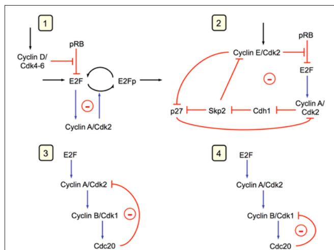
FIGURE 6 | The Cdk network driving the mammalian cell cycle contains multiple oscillatory circuits (Gérard and Goldbeter, 2009). Four circuits containing negative feedback loops are capable of generating sustained oscillations in the model for the mammalian cell cycle. Cyclin A/Cdk2 is present in the four circuits, each of which can generate on its own sustained oscillations. In circuits 1 and 2, oscillations can occur in the absence of cyclin B/Cdk1, which is responsible for the entry of cells into mitosis. Oscillations in Cdk2, which controls DNA replication, occur in these circuits without any peak in Cdk1, a phenomenon known as endoreplication (see Figure 7). In circuits 3 and 4, mitotic oscillations involving repetitive activation of cyclin B/Cdk1 can occur, based on a negative feedback exerted via the protein Cdc20, which allows the degradation of either cyclin A or cyclin B. In physiological conditions, all four oscillatory circuits synchronize to produce the ordered, repetitive activation of the different modules forming the Cdk network that drives the mammalian cell cycle (see Figure 2A).
