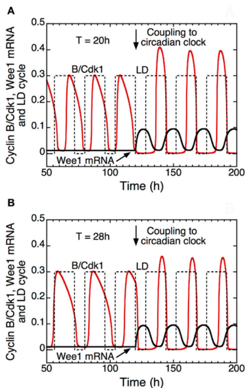
FIGURE 11 | Entrainment of the mammalian cell cycle by the circadian clock (Gérard and Goldbeter, 2012a). The curves show the time evolution of cyclin B/Cdk1 (in red), total Wee1 mRNA (in black) and the light/dark (LD) cycle (dashed line) in the absence ( t < 120 h) or in the presence ( t > 120 h) of coupling between the detailed model for the Cdk network and the model for the circadian clock in mammals (Leloup and Goldbeter, 2003). From t = 120 h on, the rate of synthesis of Wee1 mRNA, v_{sw} , that depends on the circadian complex protein CLOCK/BMAL1, passes from 0 to 0.1 \mu\text{M}\cdot\text{h}^{-1} . Starting from an autonomous cell cycle period of 20 h in (A) or 28 h in (B), the coupling through Wee1 that starts in t = 120 h elicits entrainment of the cell cycle period to a period of 24 h. In the model, the LD cycle is defined by an increase of the rate of transcription of the Per gene during the light (L) phase (see Leloup and Goldbeter, 2003; Gérard and Goldbeter, 2012a for further details). Upon entrainment, the peak of activity of cyclin B/Cdk1 occurs at the end of the L phase, which corresponds to the experimental observations (Bjarnason et al., 1999). Parameter values are the same as in Figure 3 in Gérard and Goldbeter (2012a).
