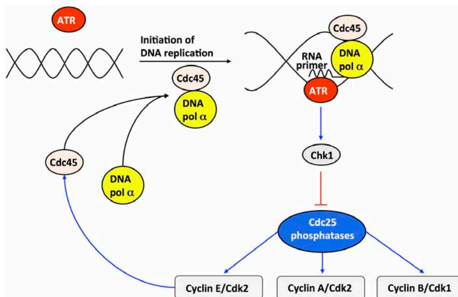
FIGURE 8 | Scheme of the DNA replication checkpoint regulated by kinases ATR and Chk1. At the G1/S transition, cyclin E/Cdk2 activates, by phosphorylation, the anchor factor Cdc45 that allows DNA polymerase \alpha to bind to DNA. Upon initiation of DNA replication, DNA polymerase \alpha synthesizes an RNA primer, which binds and activates the kinase ATR. The active form of ATR activates, by phosphorylation, the kinase Chk1. Once activated, Chk1 inhibits, by phosphorylation, the phosphatases Cdc25 responsible for the activation of cyclin E/Cdk2, cyclin A/Cdk2, and cyclin B/Cdk1. The inhibition of cyclin E/Cdk2 and cyclin A/Cdk2 during DNA replication creates a checkpoint, which limits the activation of Cdc45 and thereby prevents excessive initiation of DNA synthesis at multiple points of
