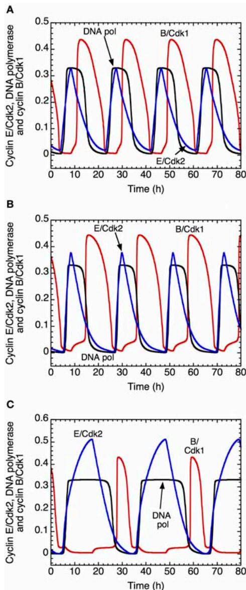
FIGURE 9 | Effect of the DNA replication checkpoint on Cdk oscillations in the detailed model for the Cdk network driving the mammalian cell cycle. The time evolution of cyclin E/Cdk2 (in blue), DNA polymerase \alpha (in black) and cyclin B/Cdk1 (in red) is shown (A) in the absence of activation of the kinase ATR driving the DNA replication checkpoint, with k_{\text{atr}} = 0 , or in the presence of low (B) or strong activation (C) of the kinase ATR, with k_{\text{atr}} = 0.01 \mu\text{M}^{-1} \cdot \text{h}^{-1} in (B) and 0.024 \mu\text{M}^{-1} \cdot \text{h}^{-1} in (C). The presence of the DNA replication checkpoint slows down the progression in the cell cycle: the period of the cell cycle clock passes from 19 h in (A), to 21.6 h in (B) and 31 h in (C). Moreover, the DNA replication checkpoint improves the separation between the phase of DNA replication, represented by the peak of DNA polymerase \alpha and the phase of mitosis, represented by the peak of cyclin B/Cdk1. Other parameter values are as in Table S2 in Gérard and Goldbeter (2009).
