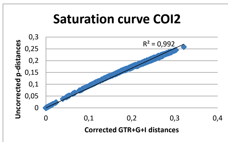
Figure 3. Substitution saturation scatter plot for the COI dataset. The graph represents the increase in GTR+I+G distances (estimated by ML), corrected for multiple nucleotide substitutions, versus the increase in p-distances between pairs of sequences. R^2 value shows the fit of the relationship to a linear regression model. In the absence of saturation, the plot should reveal a linear increment of corrected in relation to uncorrected distance. Once substitution saturation is achieved, the plot should reach a plateau.
