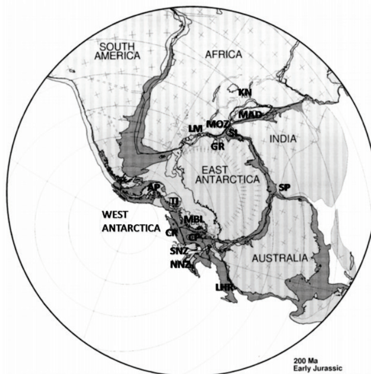
Figure 27. Reconstruction of Gondwana 200 Ma. Continents are indicated with coastlines and 2000 m isobaths. Tick marks are a 5° grid based on the present-day latitude and longitude for the continental fragments. AP, Antarctic Peninsula; CP, Campbell Plateau; CR, Chatham Rise; KN, Kenya; LHR, Lord Howe Rise; LM, Lebombo Monocline; MAD, Madagascar; MBL, Marie Byrd Land; MOZ, Mozambique; NNZ, North New Zealand; SL, Sri Lanka; SNZ, South New Zealand; SP, Shillong Plateau; TI, Thurston Island. Figure modified from Lawver et al. (1992).
