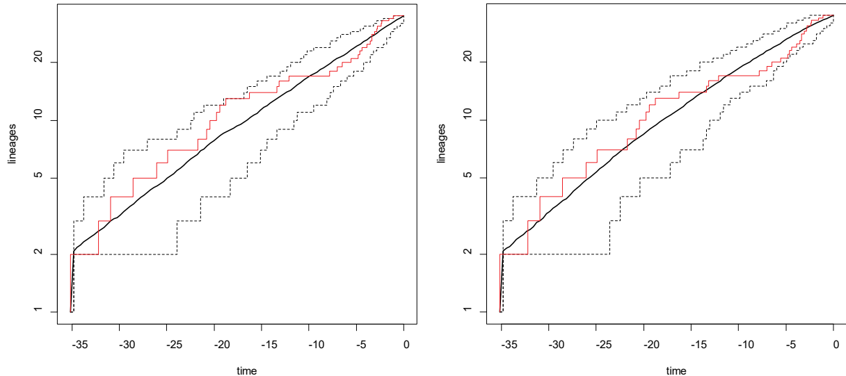
Appendix S6 -A. Lineage diversification through time plot of the Antarctic iphimeriid clade, generated with the dated tree from the BEAST analysis (in red). Dashed lines represent the 95 % confidence interval of lineage diversification simulated 100 times under a BD (left; \lambda = 0.135 and \mu = 0.06 ) and a PB (right; \lambda = 0.098 ) model, and assuming a sampling fraction of 50 %.
