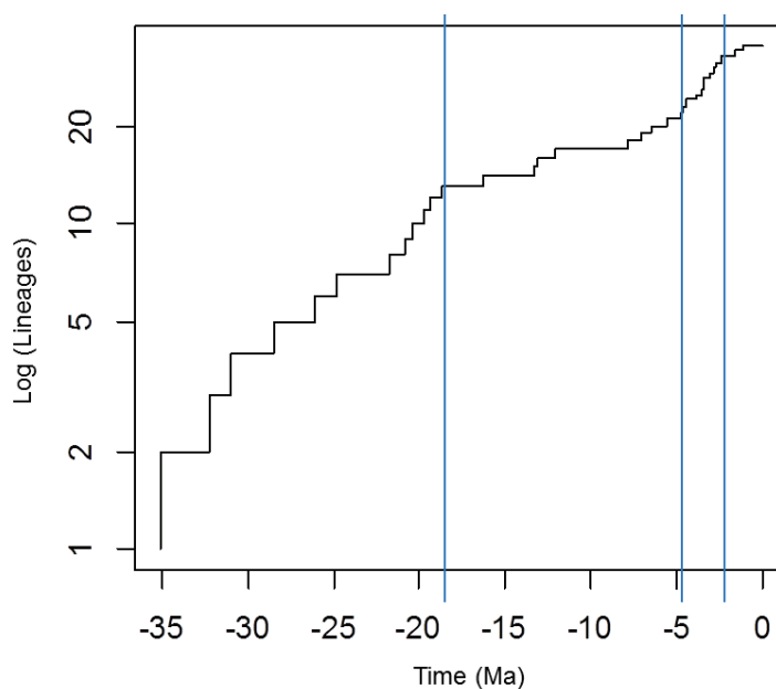
Figure 5. Rate shifts under the Yule4rate model represented on the lineage-through-time plot.
