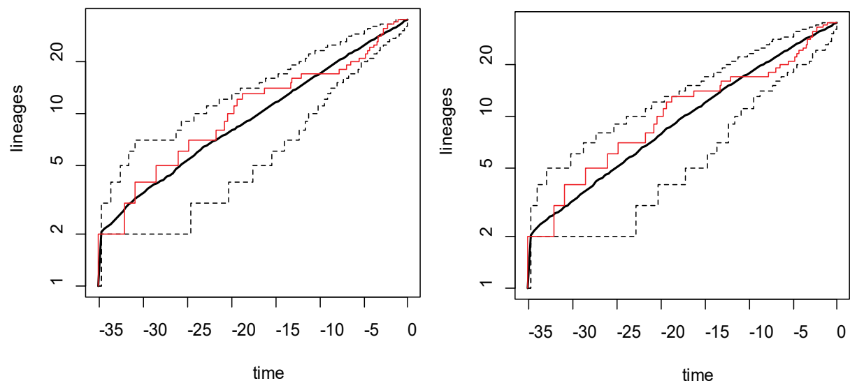
Appendix S6 -B. Lineage diversification through time plot of the Antarctic iphimeriid clade, generated with the dated tree from the BEAST analysis (in red). Dashed lines represent the 95 % confidence interval of lineage diversification simulated 100 times under a BD (left; \lambda = 0.085 and \mu = 0.008 ) and a PB (right; \lambda = 0.08 ) model, and assuming a sampling fraction of 79 %.
