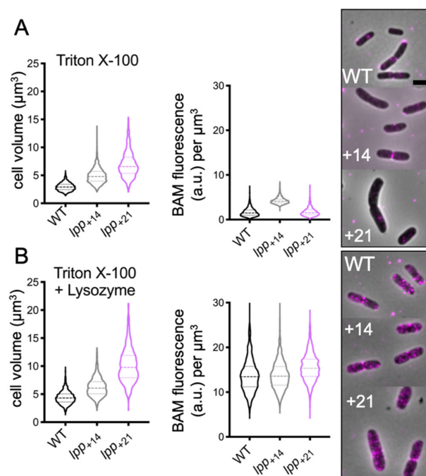
Figure 6. E. coli wild-type cells and its enlarged periplasmic derived mutants immunolabelled with αBAM. Violin plots of the BAM concentration of the wild-type MG1655 (WT, black), Lpp+14 (grey) and Lpp+21 (pink). After the peptidoglycan permeabilization (TL), the BAM signal increases about 3-fold amongst all the strains. The BAM signal is lower in cells with undigested peptidoglycan compared to the cells treated with lysozyme, irrespective of the enhanced distance between OM and PG. The cells were grown in rich medium at 37 °C. The antibodies were used in 1:500. A: wild-type n = 2062 ; Lpp+14 n = 1709 ; Lpp+21 n = 1991 . B: wild-type n = 1697 ; Lpp+14 n = 1132 ; Lpp+21 n = 1141 .
