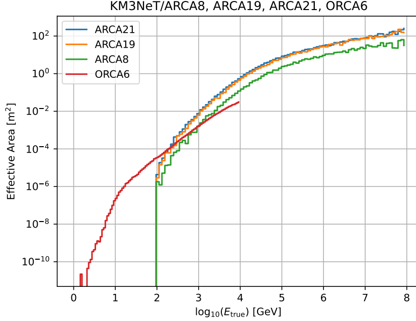
Figure 4. The effective area as a function of the true energy for muon neutrinos of the ARCA8, ARCA19 and ARCA21 detectors at the Galactic Centre declination, and the ORCA6 detector weighting declination bins according to the fractional time the source spends in each bin. The effective areas are computed after the application of the event selection.
