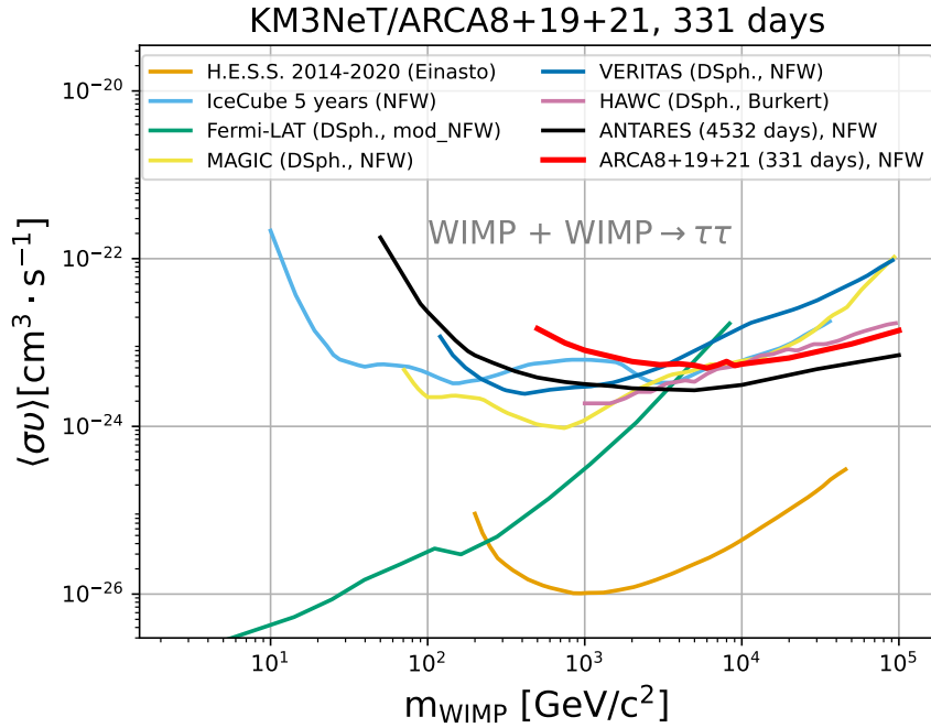
Figure 6. 90% CL upper limits on the thermally-averaged WIMP annihilation cross section, \langle\sigma v\rangle , as a function of the WIMP mass for the \tau^+\tau^- annihilation channel obtained with the ARCA8-21 data set along with results obtained by other experiments [8, 10, 14–18].
