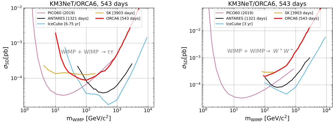
Figure 7. 90% CL upper limits on the spin-dependent WIMP-nucleon cross section as a function of the WIMP mass for the \tau^+\tau^- (left) and W^+W^- (right) annihilation channels. The red lines show the results obtained in this analysis, whereas the other lines show the upper limits obtained by IceCube [11, 12], ANTARES [9] and Super-Kamiokande [13]. The PICO-60 limit [5] is obtained from the direct search of WIMP-nucleon scatterings and as such is independent of the annihilation channel considered.
