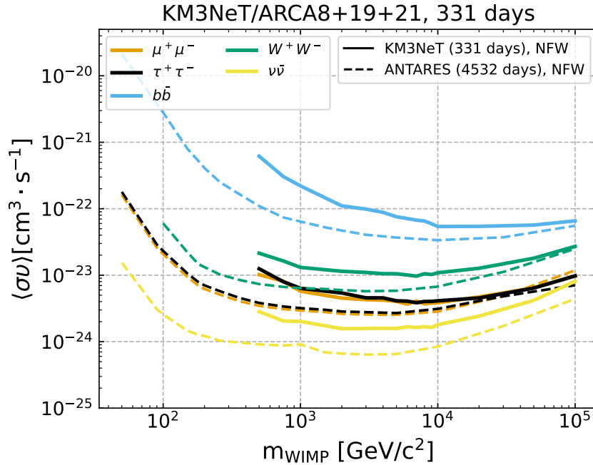
Figure 5. 90% CL upper limits on the thermally-averaged WIMP annihilation cross section, \langle\sigma v\rangle , as a function of the WIMP mass for each of the five annihilation channels, obtained with the ARCA8-21 data set (full lines) and with the ANTARES 4532 day data set (dashed lines) [8].
