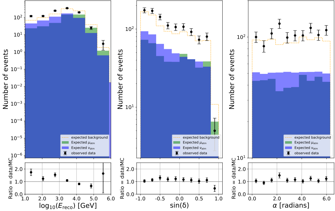
Figure 3. The distributions of the reconstructed energy (left), sine of the declination (middle) and the right ascension (right) in ARCA21 after the application of the event selection. The distributions of data events are shown as black dots, the expected distribution of atmospheric muons is shown in green and the simulation of atmospheric neutrinos is shown in blue, while the dashed line is the total MC expected background. The ratio plot shows the ratio between the number of data events and the total MC background in each bin.
