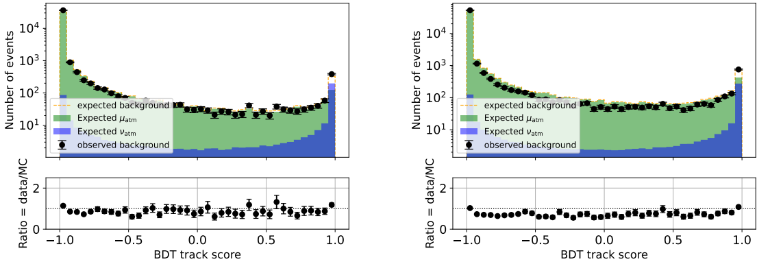
Figure 2. BDT score distributions of data events and the MC background expectation prior to the application of the final event selection, shown for the ARCA19 detector (left) and ARCA21 (right). Black dots indicate data events, the atmospheric muon simulation is shown in green, the atmospheric neutrino simulation in blue and the dashed line indicates the total number of simulated background events. The ratio plot compares the number of data events in each bin to the total number of expected background events from simulations. The final selection places a cut on the BDT score at 0.95, for both the ARCA19 and ARCA21 detectors.
