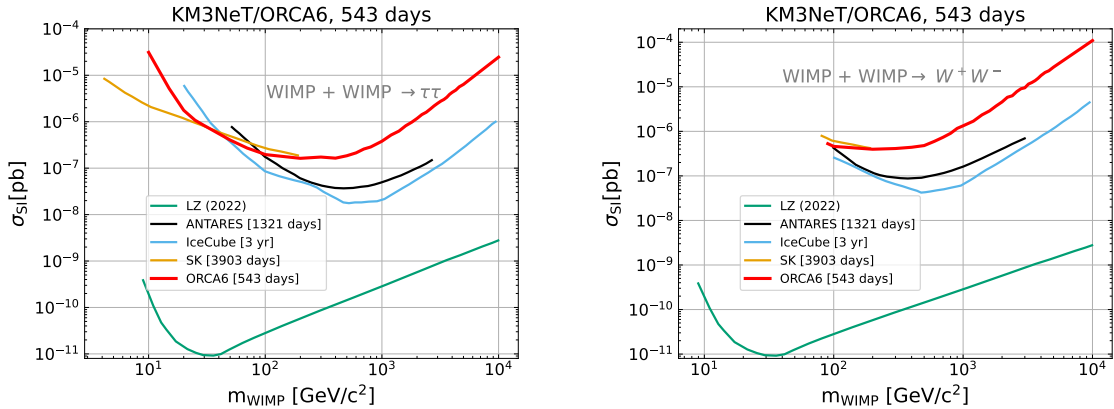
Figure 8. 90% CL upper limits on the spin-independent WIMP-nucleon cross section as a function of the WIMP mass for the \tau^+\tau^- (left) and W^+W^- (right) annihilation channels. The red lines show the results obtained in this analysis, whereas the other lines show the upper limits obtained by IceCube [11, 12], ANTARES [9] and Super-Kamiokande [13]. The LZ [4] limit is obtained from a direct search and as such is independent of the annihilation channel.
