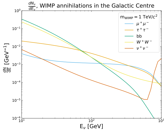
Figure 1. Number of muon neutrinos produced in one WIMP-pair annihilation in the Galactic Centre as a function of the neutrino energy. The curves are shown for a WIMP mass of m_{\text{WIMP}} = 1 \text{ TeV}/c^2 annihilating into muons, taus, b-quarks, W bosons and directly to neutrinos.
