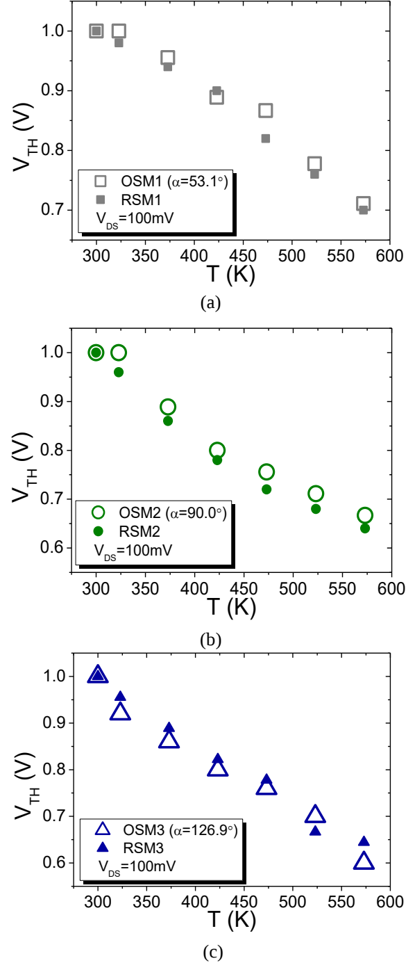
Fig.3 Curves of all SOI MOSFET V_{TH} as a function of temperature, regarding different \alpha angles of the OSM [ 53.1^\circ (Fig. 3.a), 90^\circ (Fig. 3.b), and 126.9^\circ (Fig. 3.c)] and their respective RSM counterparts.
