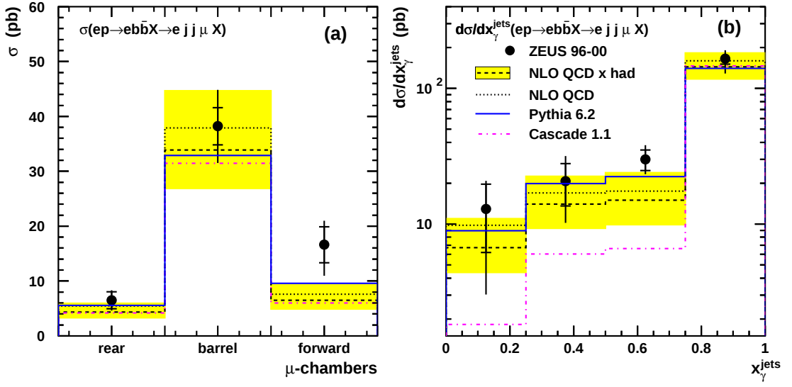
Figure 4: Cross sections for muons coming from b decays in dijet events with p_T^{\text{jet}_1} > 7, p_T^{\text{jet}_2} > 6 \text{ GeV} , \eta^{\text{jet}_1}, \eta^{\text{jet}_2} < 2.5 , 0.2 < y < 0.8 , Q^2 < 1 \text{ GeV}^2 passing the selection of Eq. (1). (a) The cross section for the forward, barrel and rear regions (defined in Eq. (1)). (b) The differential cross section as a function of x_{\gamma}^{\text{jets}} . The data (points) are compared to the predictions of NLO QCD (dotted line: parton-level jets; dashed line: jets corrected to the hadron level). The full error bars are the quadratic sum of the statistical (inner part) and systematic uncertainties. The band around the NLO prediction represents the variation on the theoretical predictions obtained by varying the b -quark mass, \mu_r and \mu_f , as explained in the text. The data are also compared to the predictions of the PYTHIA (solid line histogram) and CASCADE (dot-dashed line histogram) Monte Carlo models.
