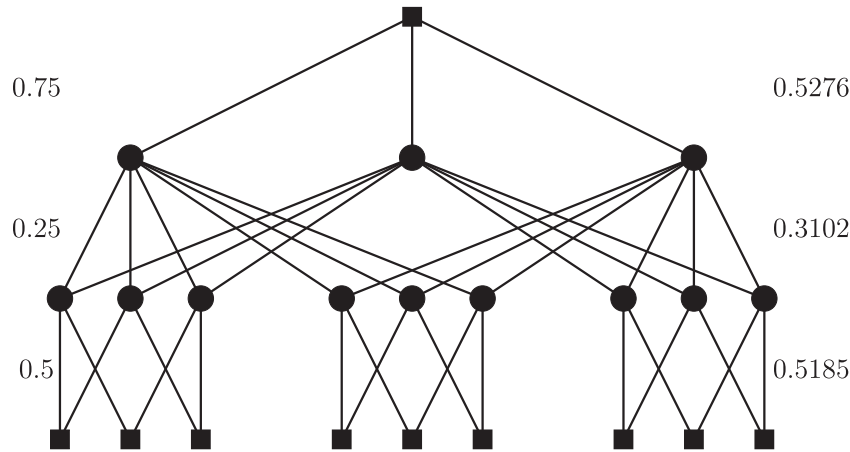
FIGURE 9 A different instance of a graph showing improvement between consecutive extended formulation levels. Numbers on the left side show the flow limits provided by MCF-2 and numbers on the right side show flow limits provided by MCF-3
