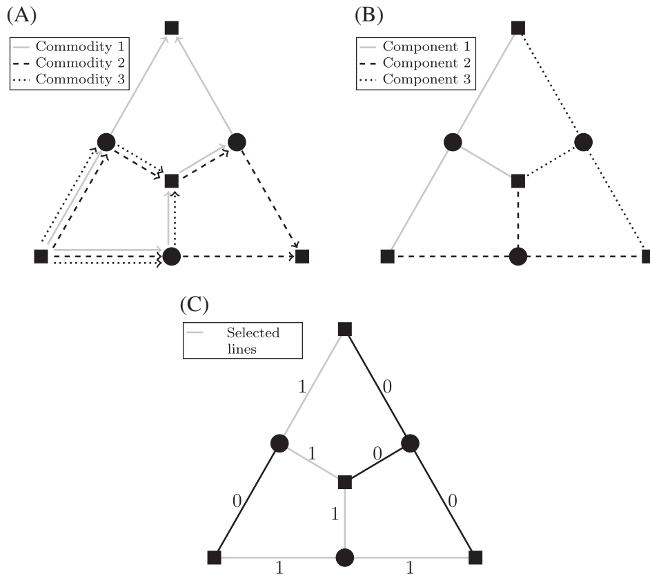
FIGURE 4 Sample solutions of instance 2C with BCR, HYP, and MCF-2 formulations. (A) Solution using BCR: for each commodity there are two paths of flow. Each path carries 0.5 units of flow. (B) Solution using HYP makes use of three components, each with weight 0.5. (C) Solution using MCF-2 in terms of edge variables y . Edges are chosen such that the flow along one outer edge is replaced by flow through the central terminal
