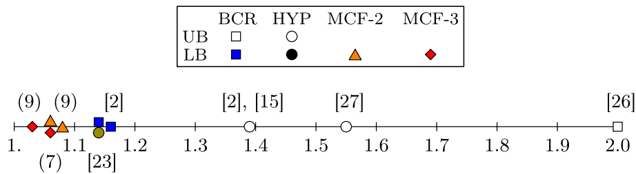
FIGURE 10 Comparison of integrality gap bounds for different formulations of STP [Colour figure can be viewed at wileyonlinelibrary.com]
