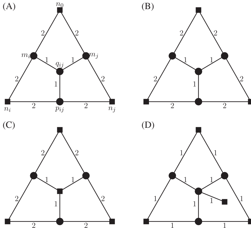
FIGURE 2 Instances of graphs based on the family of graphs proposed by Goemans [13]. (A) Segment of a graph belonging to the family of graphs proposed by Goemans. (B) An instance for N = 2 with 3 terminals. (C) A modified instance with an additional “central” terminal node. (D) A modified instance with an additional terminal node attached to the central vertex [9]
