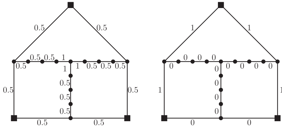
FIGURE 6 The MCF-2 (left) and MCF-3 (right) solutions in terms of y variables to the instance presented in Figure 5. The higher level formulation eliminates flow joining and splitting at the center node
