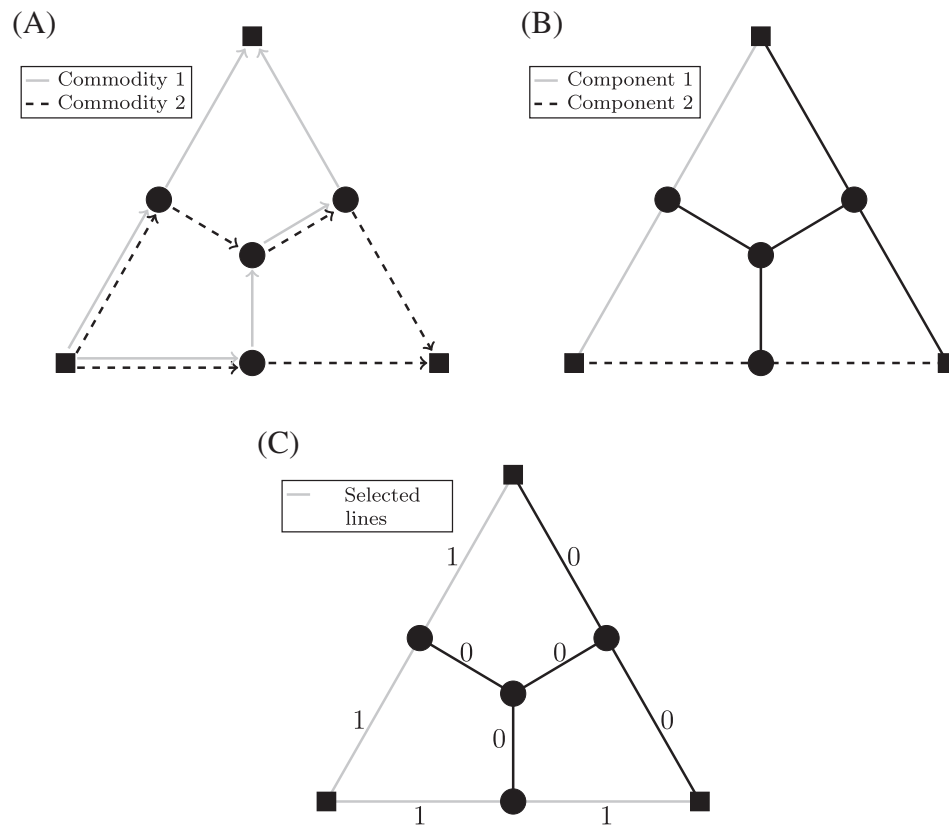
FIGURE 3 Sample solutions of instance 2B with BCR, HYP, and MCF-2 formulations. (A) Solution using BCR: for each commodity there are 2 paths of flow, one along the outer edges and the other through the center. Each path carries 0.5 units of flow. (B) Solution using HYP: two components joining the terminals along outer edges are chosen, one for each commodity. (C) Solution using MCF-2 in terms of edge variables y . Only four outer edges are picked, such that they provide a solution similar to HYP.
