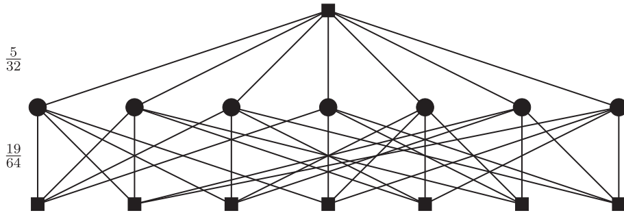
FIGURE 7 Skutella's graph, an example of 8/7 integrality gap for HYP formulation. All edges have weight 1. Numbers on the left side show the flow limits provided by our hierarchy of extended formulations
