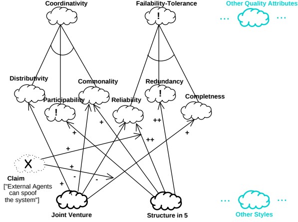
Fig. 7. Partial Evaluation for Organizational Styles
