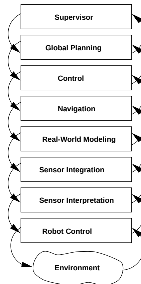
Fig 3. Mobile Robot Layered Architecture [Sim97]
