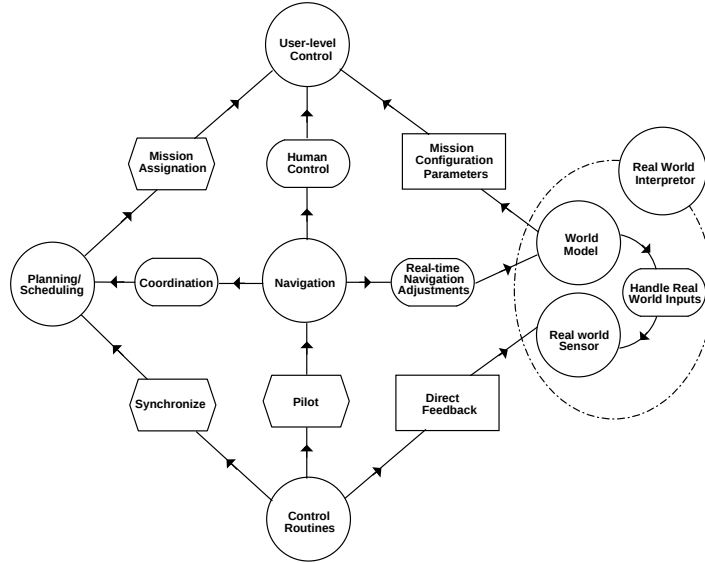
Fig 6. A structure-in-5 mobile robot architecture.
