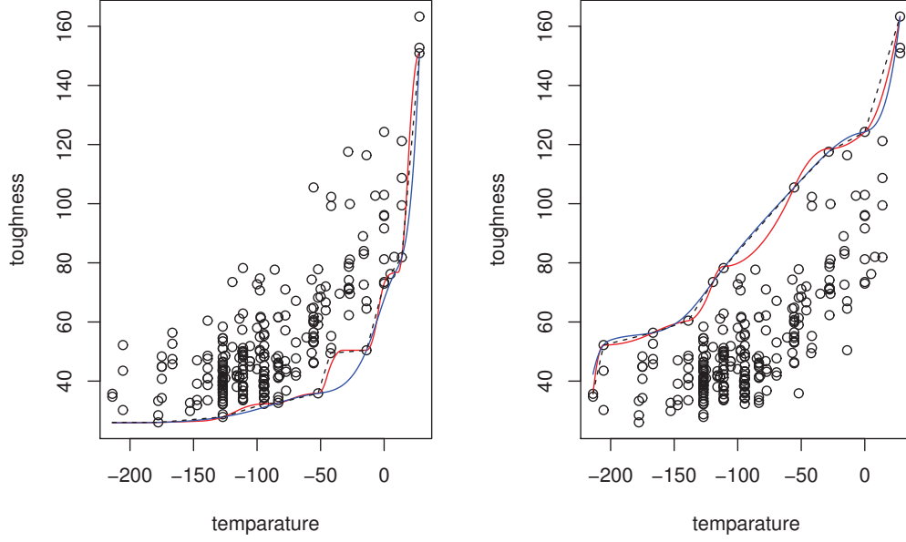
Figure 5: Scatterplot of the 254 nuclear reactors data, with three frontier estimates: LFDH (dotted black), QS-A (solid red) and CS-A (solid blue). From left to right, the estimates for the lower and the upper support boundaries.
