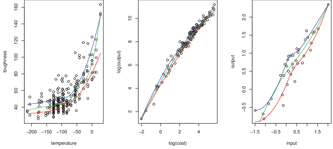
Figure 1: Scatterplots of three real datasets with the quartile curves in each plot. The three regression quantile curves are estimated by the method of He and Shi (1998).
