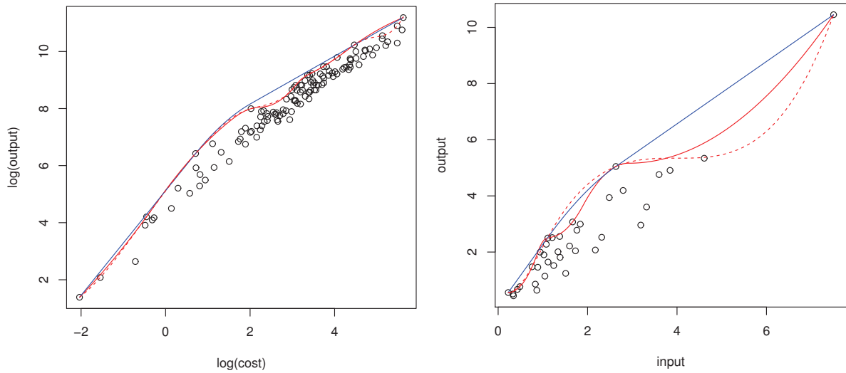
Figure 6: Scatterplots of the 123 American electric utility companies' data and the 37 European Air Controllers' data with three estimates of the efficient extremity in each plot: QS-A (solid red), CS-A (dotted red) and QS-C (solid blue)
