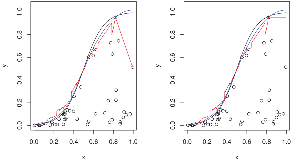
Figure 4: The problem of the local linear frontier estimator (left panel) and the illustration of its improved version (right panel)-LL (red curve), QS-A (blue curve) and the true frontier (black curve)
