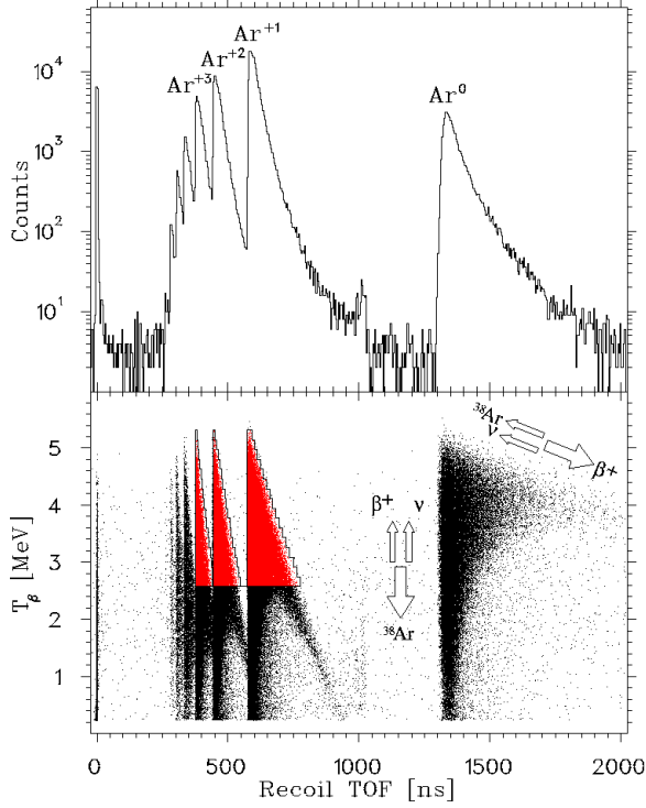
FIG. 2: (color online) Bottom: Scatter plot of recoil TOF vs. T_\beta with one dot shown for each of 500 000 events. The suppressed back-to-back lepton emission produces longer recoil TOF. The E field separates the Ar charge states. The analysis cuts are shown. Top: TOF projections of the 2D scatter plot. The 0.1% background at \text{TOF} \approx 1020 ns is from \beta 's scattering off the MCP into the \beta telescope and can be rejected kinematically.
