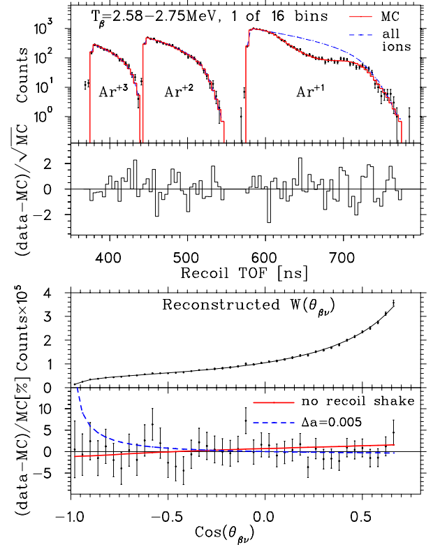
FIG. 3: (color online) Top: lowest of 16 T_\beta bins for the MC fit to the \text{Ar}^{+1,+2,+3} data, and residuals. The confidence level for the entire fit is 52%. Data has been binned to show sensitivity to a . Fits are done with 4 ns bins. The dip in \text{Ar}^{+1} is from the finite MCP size: the dashed curve has an artificially larger MCP collecting all ions. Bottom: Fit to reconstructed angular distribution, showing residuals. Also shown are the effect of a change in a by 0.005, and the effect of recoil energy-dependent shakeoff.
