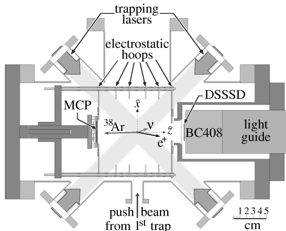
FIG. 1: Top view of the 2 nd MOT apparatus with the recoil and \beta detectors.
