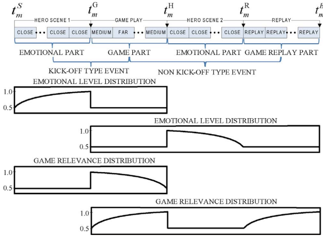
Fig. 4. Game relevance and emotional level are assigned as a function of clips view-types, where t_m^S, t_m^E are the starting and ending times of the m th segment, and t_m^G, t_m^H, t_m^R are starting times of its game play part, hero scene part, and replay part, respectively.
