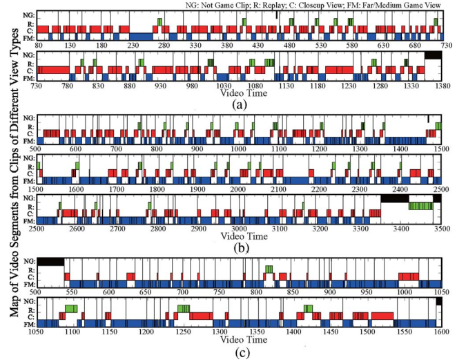
Fig. 6. Results of view-type based video segmentation for the soccer, basketball, and volleyball videos in our experiments. (a) Volleyball (first set). (b) Soccer (first half). (c) Basketball (first quarter).
