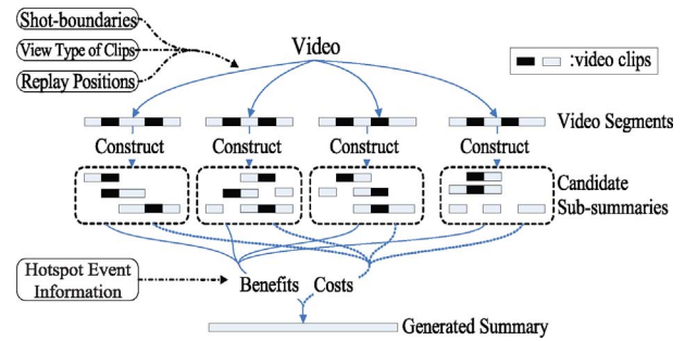
Fig. 1. Summarization in a divide-and-conquer paradigm.
