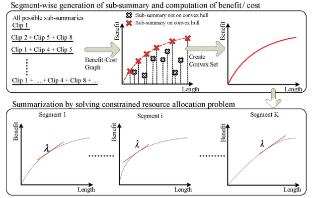
Fig. 5. Working flow in our summarization framework.
