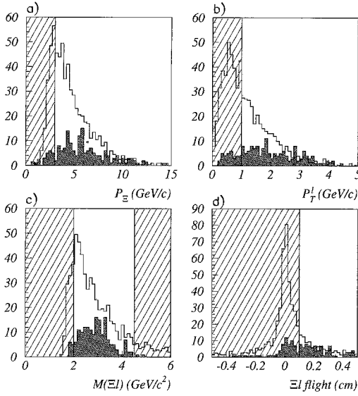
Fig. 4. Distributions of the variables, from simulated events, to select semileptonic decays of B-baryons. (a) \Xi^\pm momentum distribution. (b) Lepton transverse momentum distribution. (c) \Xi - \ell mass distribution. (d) Algebraic distance between the \Xi - \ell vertex and the primary vertex measured in the direction of the momentum of the \Xi - \ell system. Events originating from a B-baryon direct semileptonic decay are shown in cross-hatched histograms; other sources are displayed in un-hatched histograms. Regions rejected by the applied selection cuts are shown inside single-hatched areas
