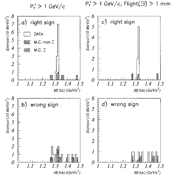
Fig. 6. \Lambda\pi mass distributions obtained with the "HT" algorithm for right-sign and wrong-sign \Xi^\pm - \ell pairs. (a, b) The lepton transverse momentum is larger than 1 GeV/c (c, d) In addition, the distance between the primary and the \Xi^\pm - \ell vertex, measured in a plane transverse to the beam axis, in the direction of the jet containing the \Xi^\pm hyperon, has to be larger than 1mm
