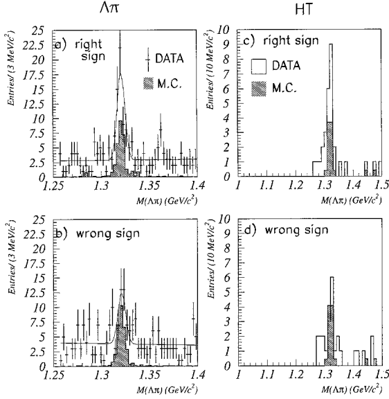
Fig. 5. Comparison between measured and expected numbers of right-sign and wrong-sign \Xi^\pm - \ell pairs. The hatched histograms represent the Monte-Carlo events, which include only the contribution from \Lambda_b and \Xi_b semileptonic decays but not the combinatorial background. The fitted curves are the sum of a first order polynomial distribution to describe the combinatorial background and of a Gaussian distribution of fixed width and central values to account for the signal
