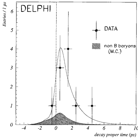
Fig. 9. Proper time distribution of the 10 right-sign \Xi^\pm - \ell^\pm events selected with P_T^l > 1 GeV/c using the “HT” algorithm. The shaded area corresponding to the expected distribution for non B-baryon events has been obtained from the Monte Carlo simulation (rate and shape)
